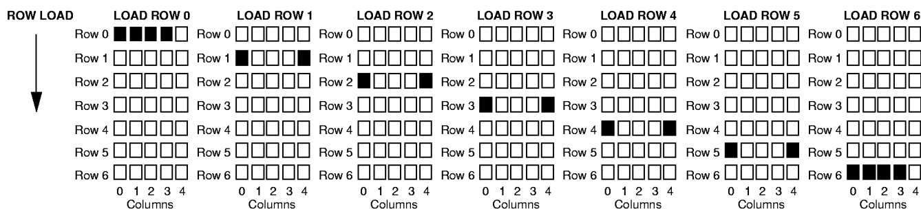
Figure 9. Row Strobing
