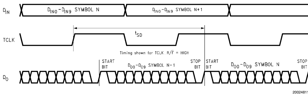
FIGURE 11. Serializer Delay
