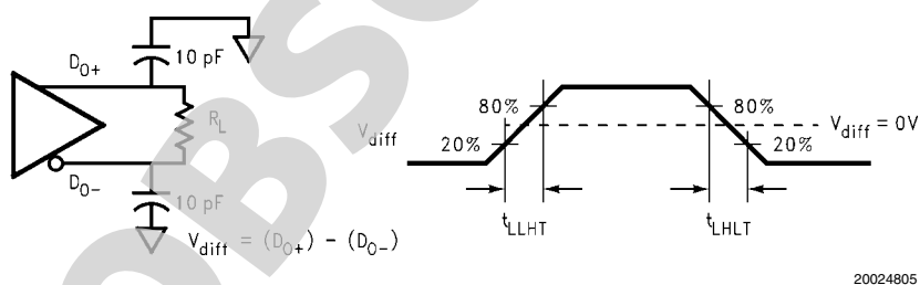
FIGURE 4. Serializer Bus LVDS Output Load and Transition Times
