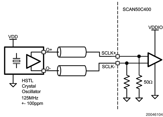
FIGURE 1. SCLK± Driven by HSTL Clock Driver / Crystals
