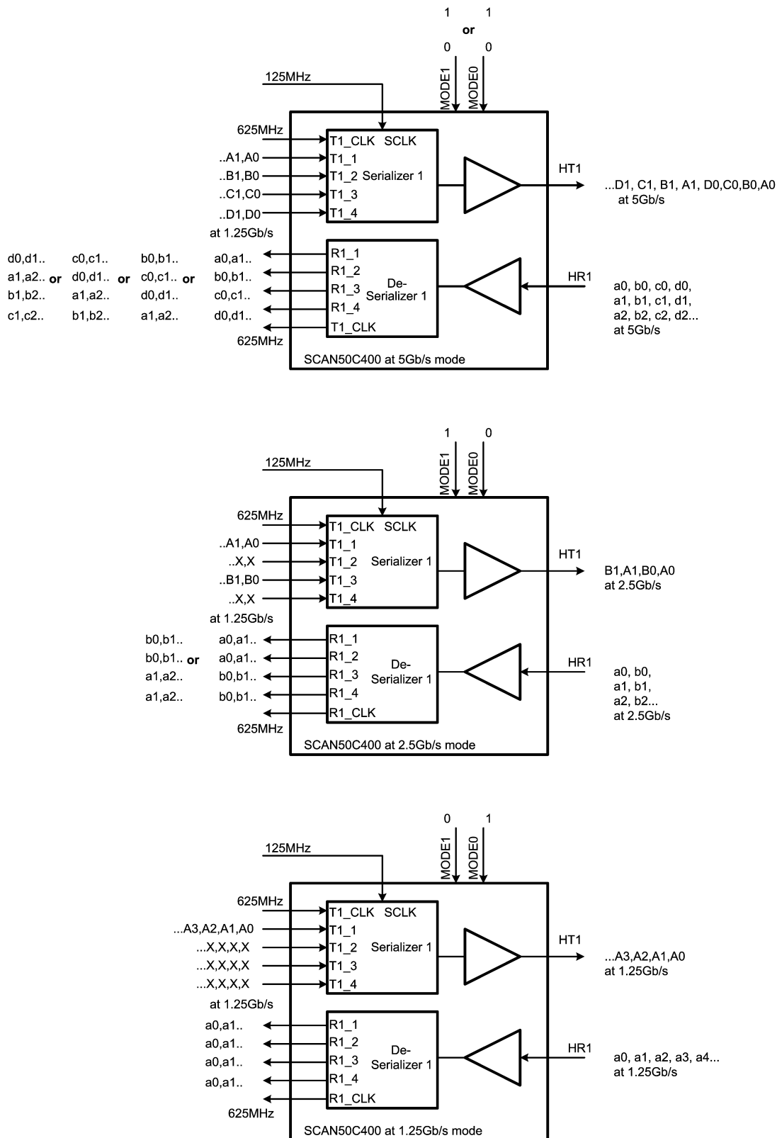
FIGURE 2. SCAN50C400 at 5, 2.5 and 1.25 Gbps Modes, Channel 1 Shown (x = don't care)
