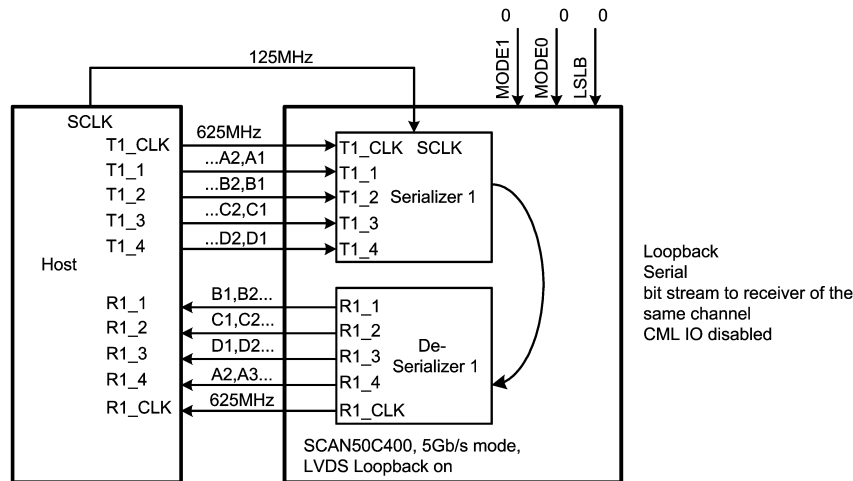
FIGURE 6. SCAN50C400 in LVDS Loopback (Channel 1 at 5 Gbps Shown)
