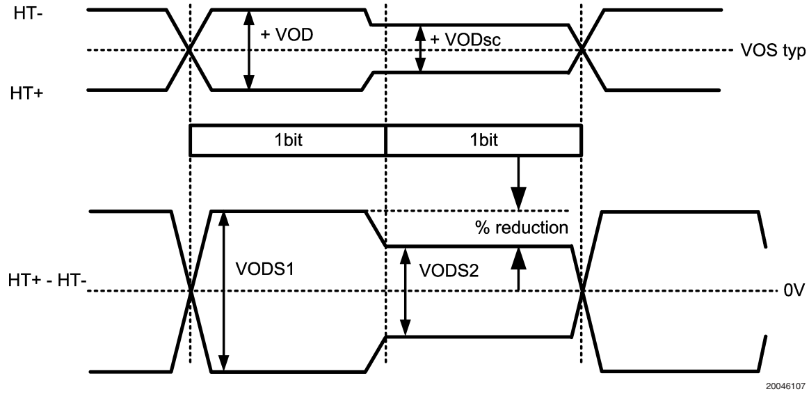
FIGURE 4. High-Speed CML Output Waveforms with signal conditioning enabled
