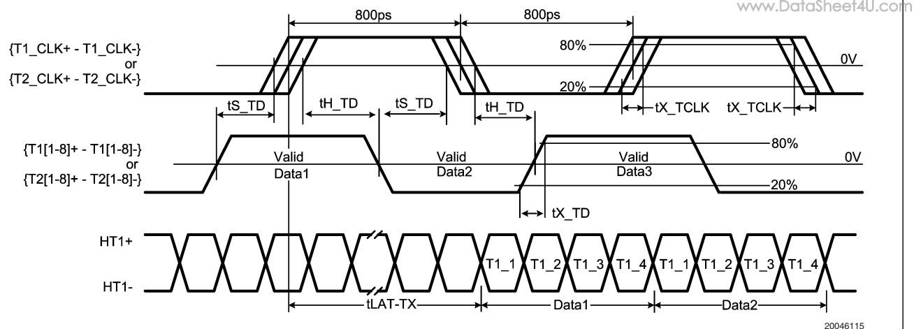
FIGURE 9. Transmit Data Timing
