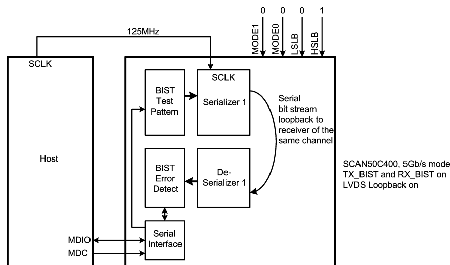
FIGURE 8. At-speed BIST Modes Used with Local Loopback
