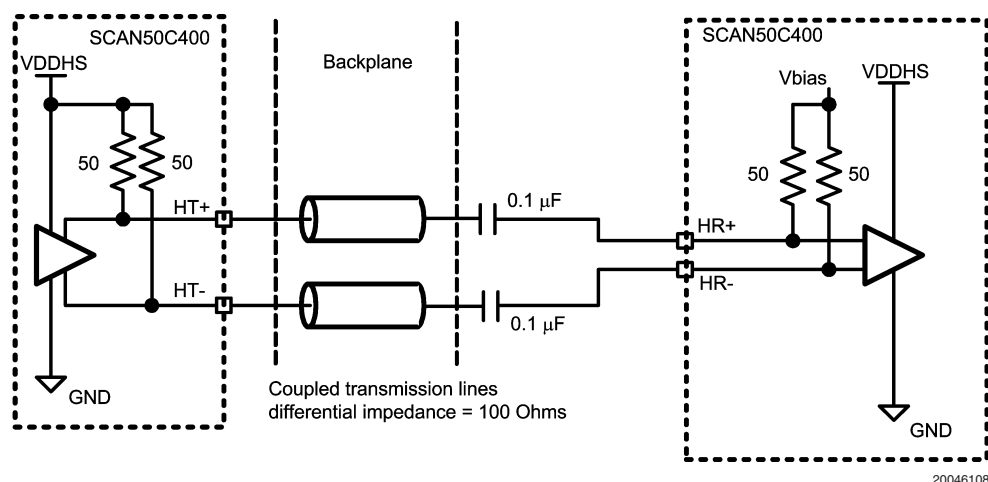
FIGURE 5. High-Speed IO, AC Coupled
