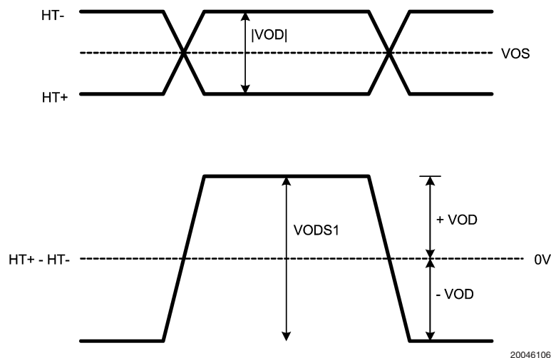
FIGURE 3. High-Speed CML Output Waveforms with de-emphasis disabled (Full VOD)
