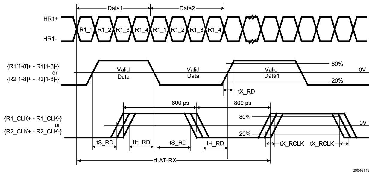
FIGURE 10. Receive Data Timing
