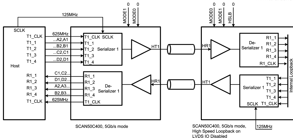
FIGURE 7. SCAN50C400 in High-Speed Loopback (5 Gbps Shown)
