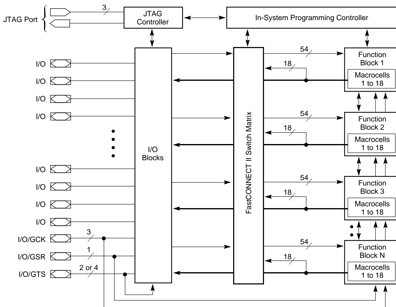
Figure 1: XC9500XV Architecture
