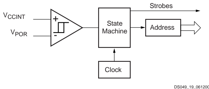
Figure 19: Configuration Controller
