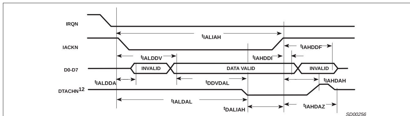
Figure 4. Interrupt Cycle Timing
