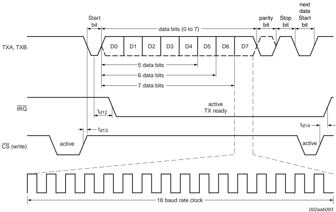
Fig 12. Transmit timing
