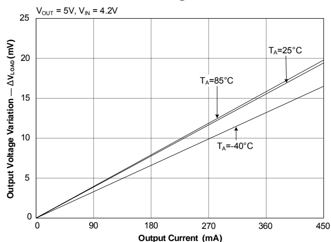
Load Regulation
