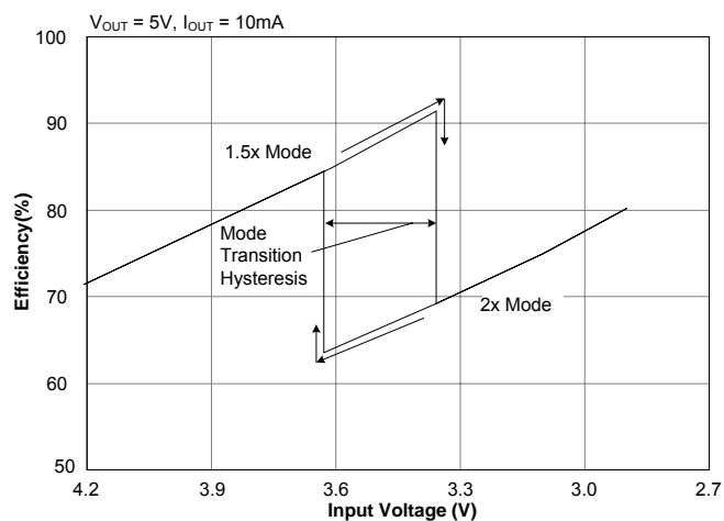
Efficiency — 10mA
