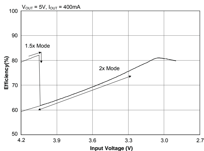
Efficiency — 400mA
