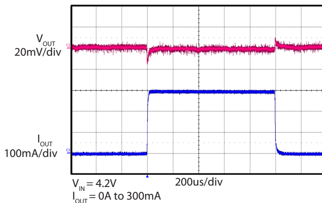
LDO2=1.8V, 0 to 300mA Load Transient
