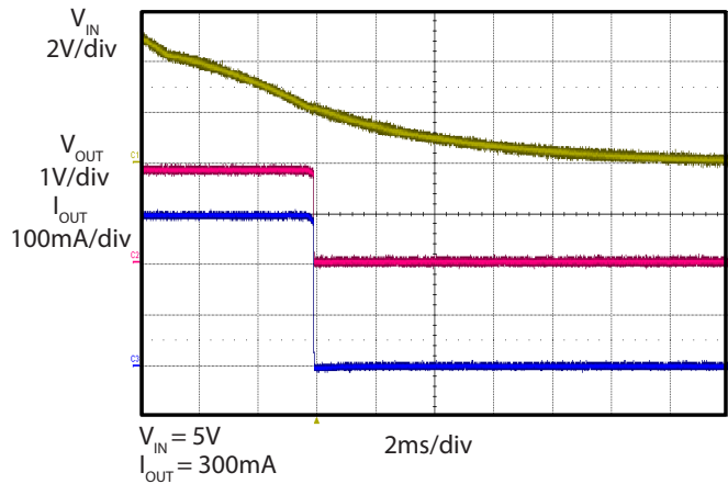
Shutdown ( V_{OUT}=1.8V )
