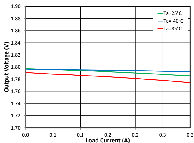
Load Regulation (Vin=4.2V, Vout=1.8V)
