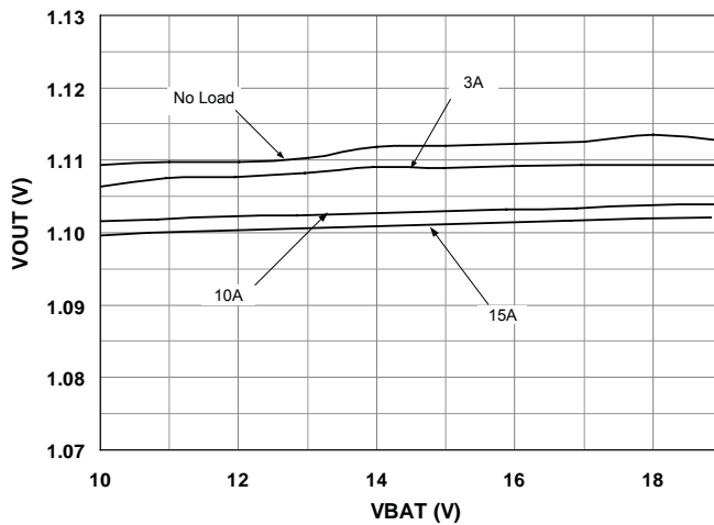
Line Regulation
