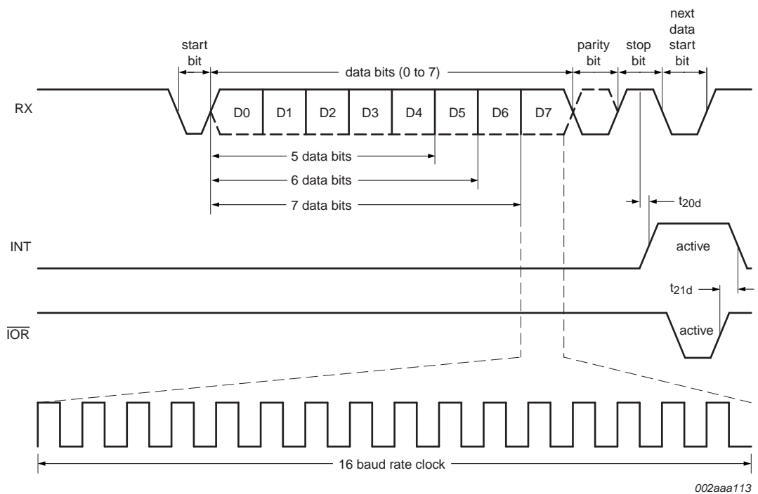
Fig 18. Receive timing
