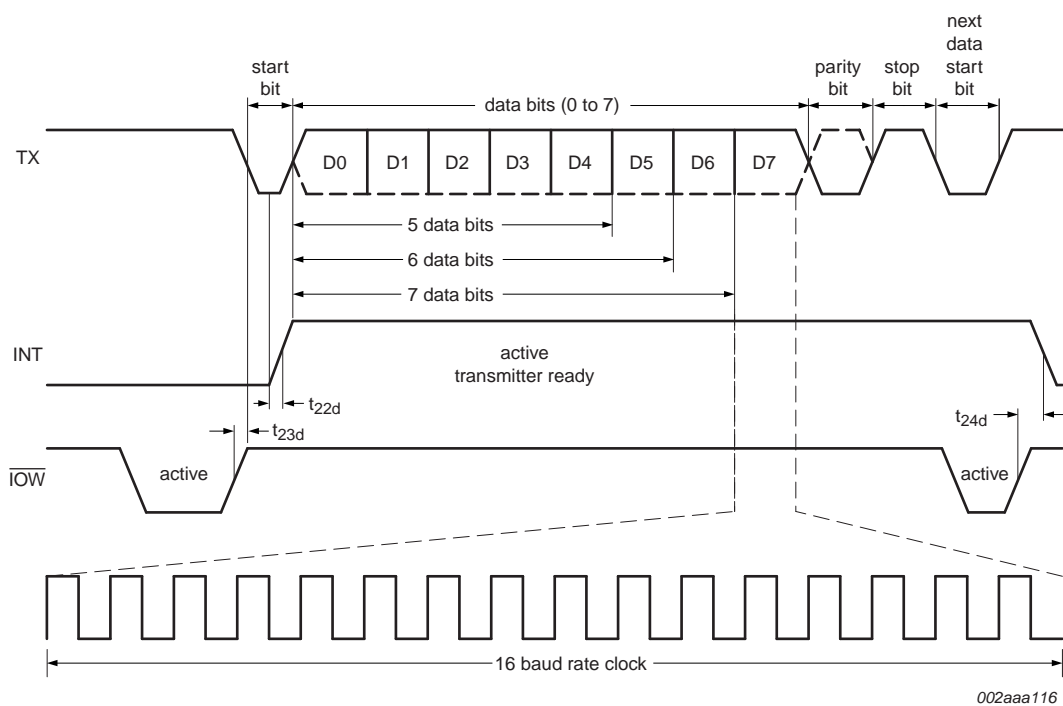
Fig 21. Transmit timing
