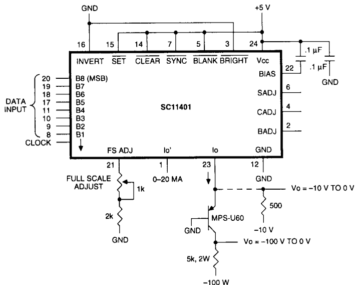
Figure 5. Non-Video Application: High speed DAC with 10 V or 100 V output swing. \overline{\text{SYNC}} and \overline{\text{BLANK}} are pulled high while \overline{\text{BRIGHT}} is low and \text{io}' is left open. This minimizes power consumption by effectively turning off the \text{io}' current sources. The SC11401 can directly drive a 500 \Omega load connected to a -10 V supply. For higher voltage swings, a high voltage PNP transistor, such as the MPS-U60 can be used, along with a 5K, 2 \Omega resistor.
