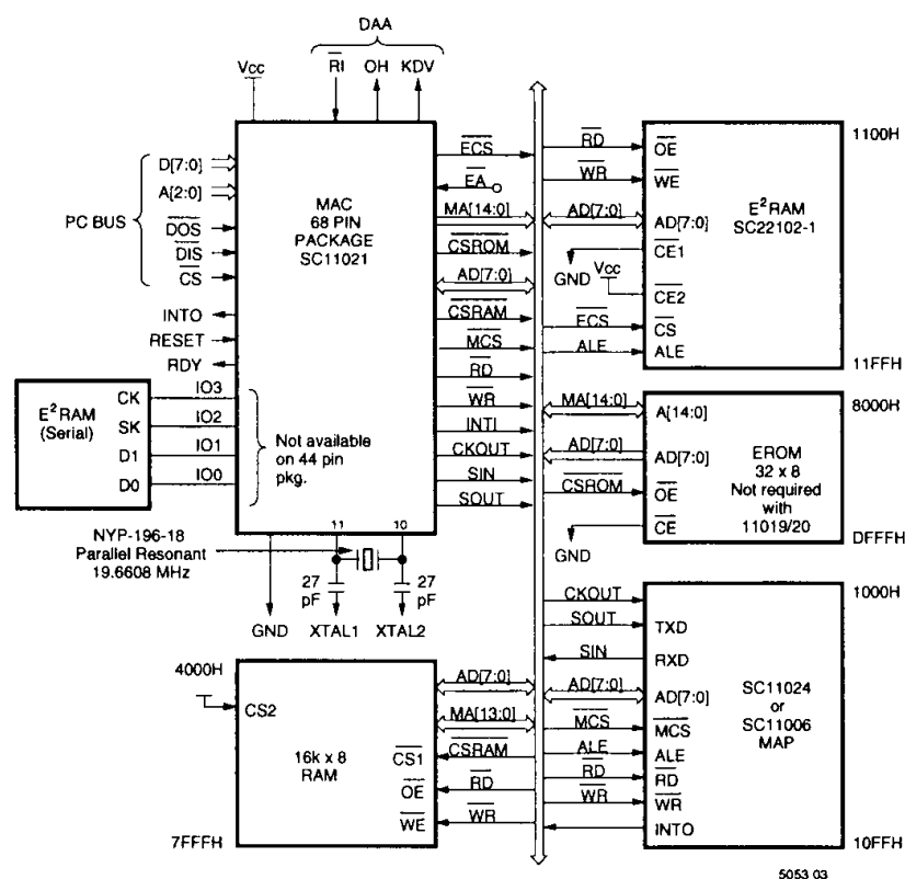
Figure 2. MAC 68 Pin Package Interfaces to E 2 PROM, ROM Map
