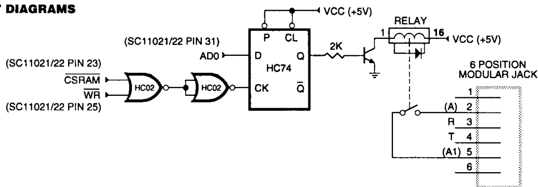
Figure 10. Circuit for Implementing &amp; J1 Command
