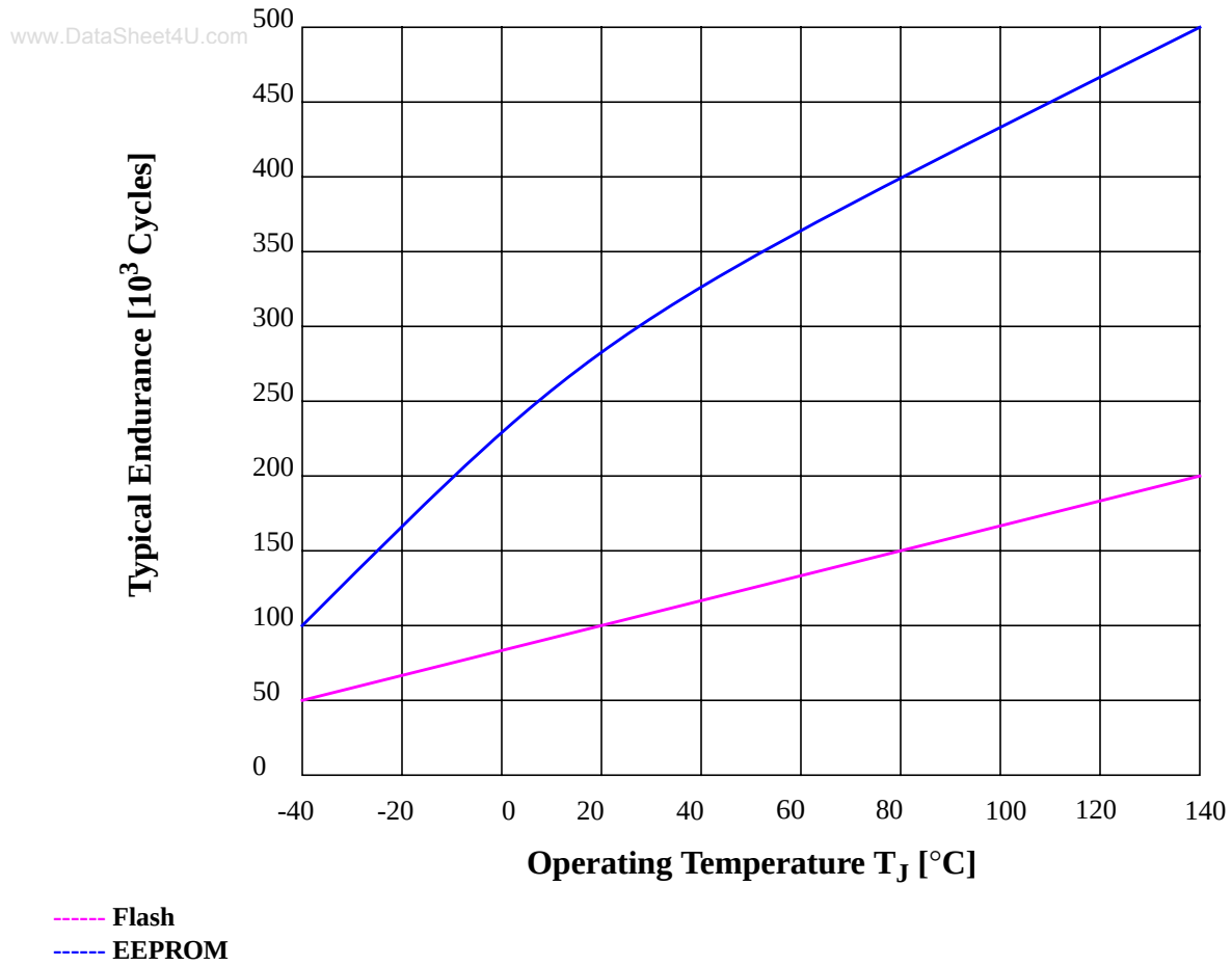
Figure A-2 Typical Endurance vs Temperature
