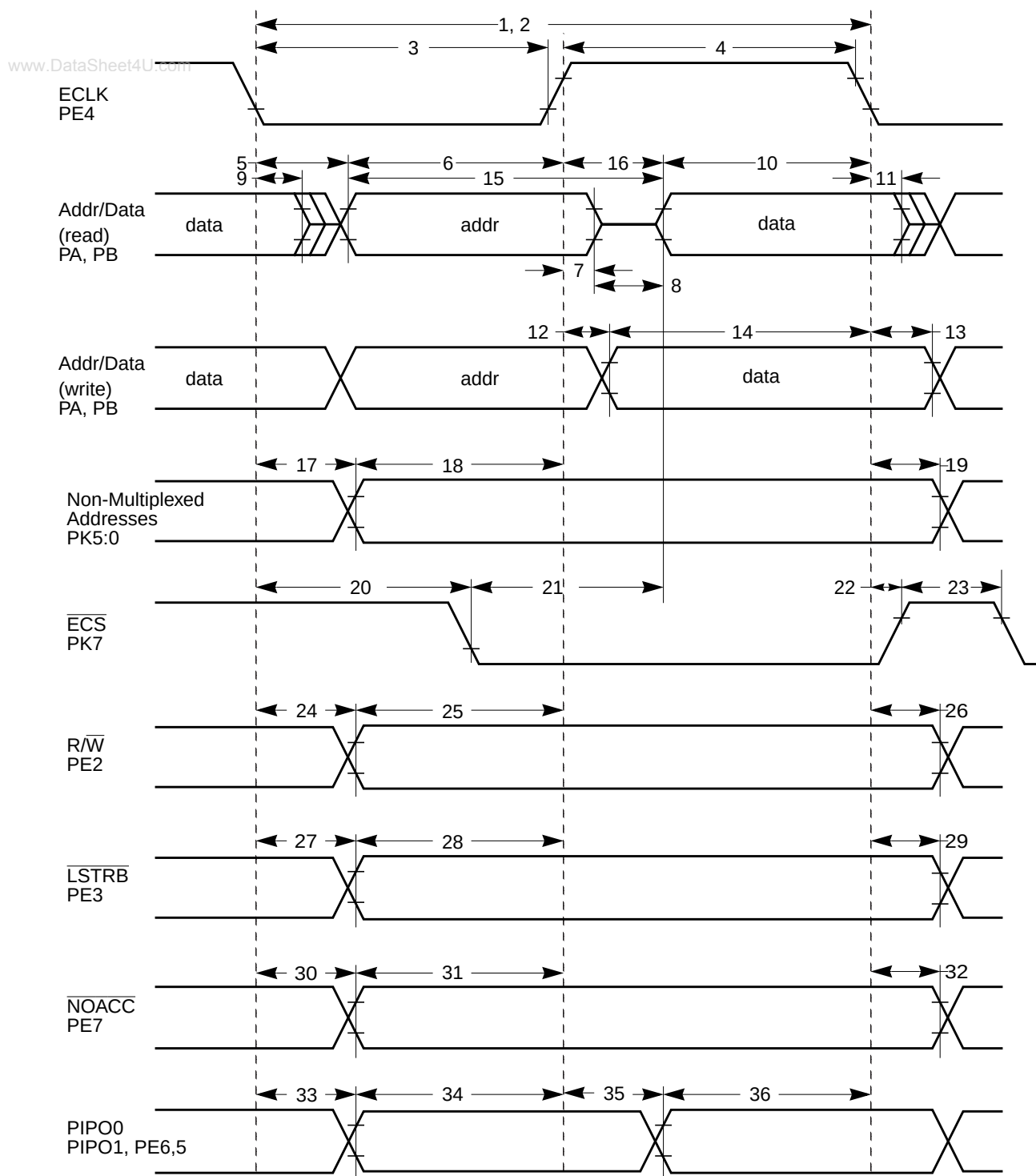
Figure A-10 General External Bus Timing
