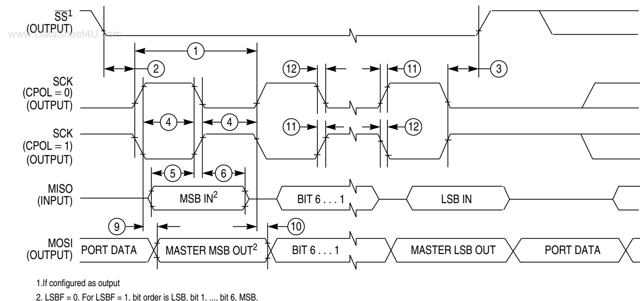
Figure A-7 SPI Master Timing (CPHA =1)
