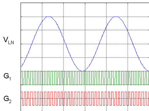
Gate pulses in permanent pulse train mode
