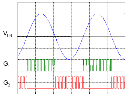
Gate pulses in synchronous pulse train mode
