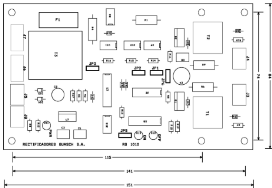
Dimensions and component situation
