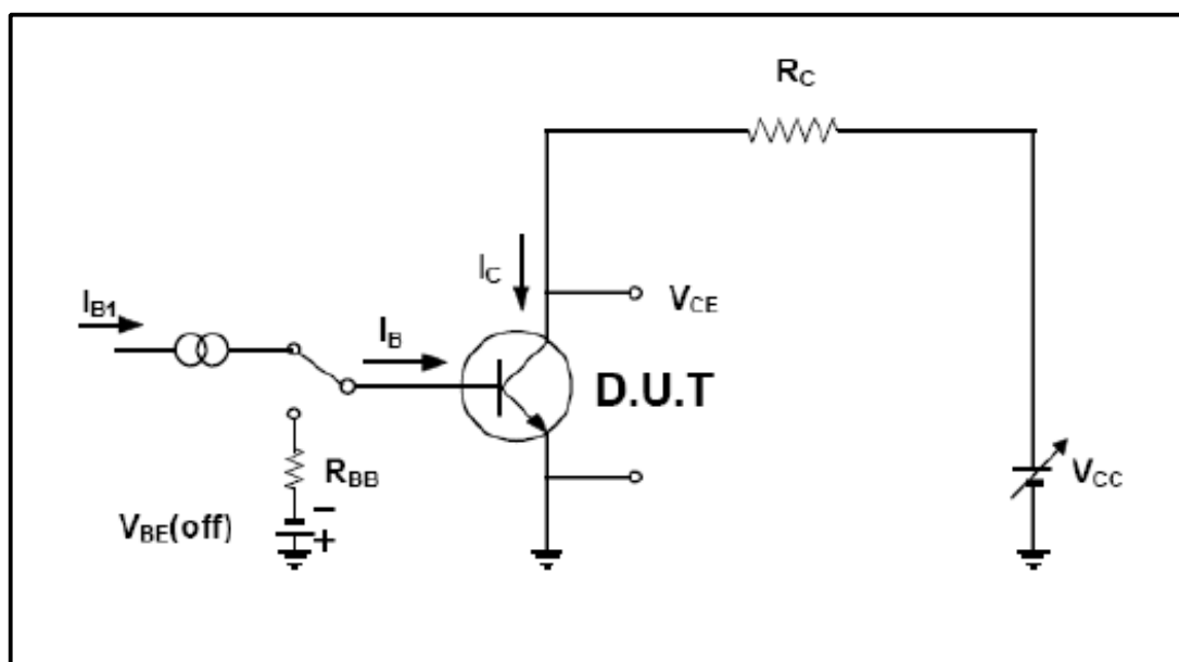
Resistive Load Switching Test Circuit
