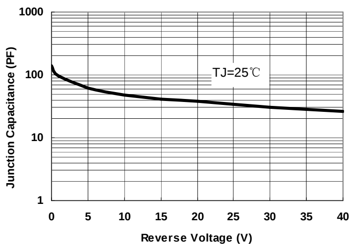
Fig.1-Typical Junction Capacitance
