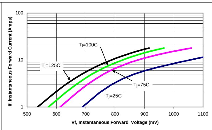
Figure 2: Typical Forward Voltage (per leg)
