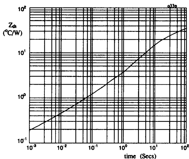
Fig 2. Transient thermal impedance characteristic per leg for SBR05 thru SBR10
