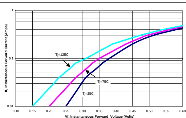
Figure 2: Typical Forward Voltage
