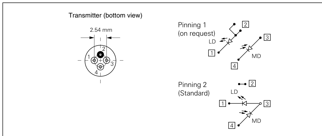
Figure 1 Transmitter
