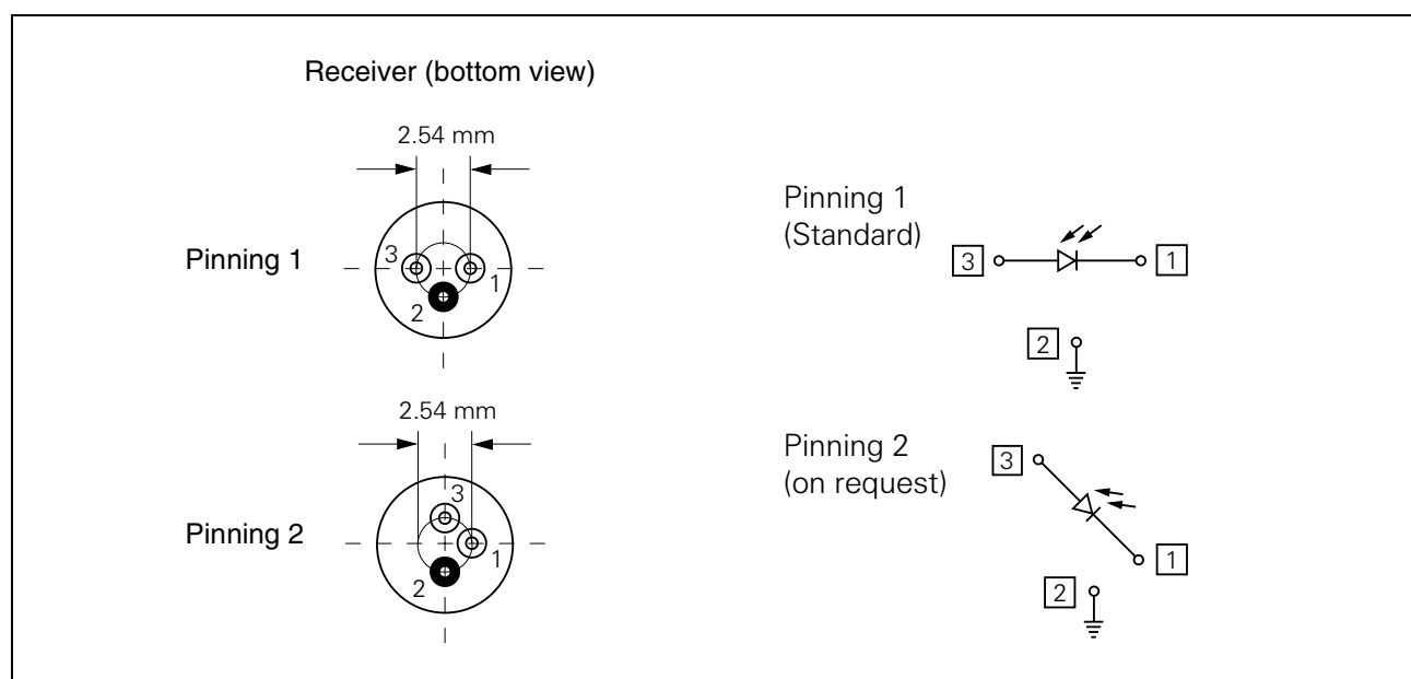
Figure 2 Receiver
