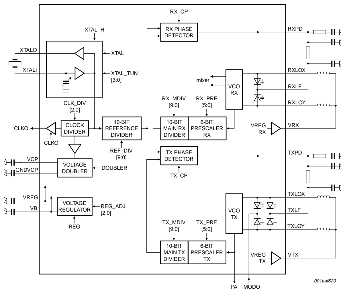
Fig 5. Synthesizer part
