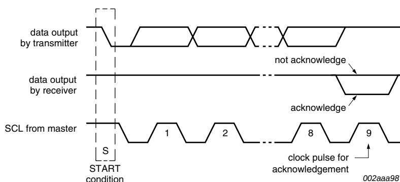
Fig 7. Acknowledgement on the I 2 C-bus
