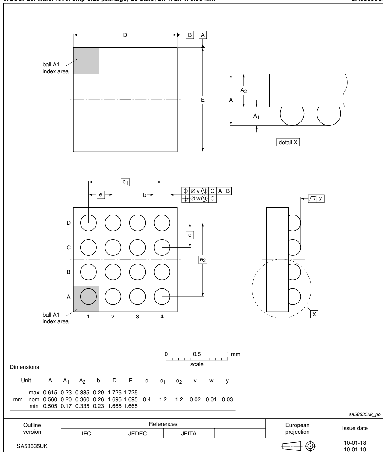
Fig 26. Package outline SA58635UK (WLCSP16)
