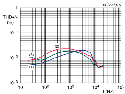
Fig 20. Total harmonic distortion-plus-noise versus frequency ( V_{DD} = 2.5 \, \text{V} )
