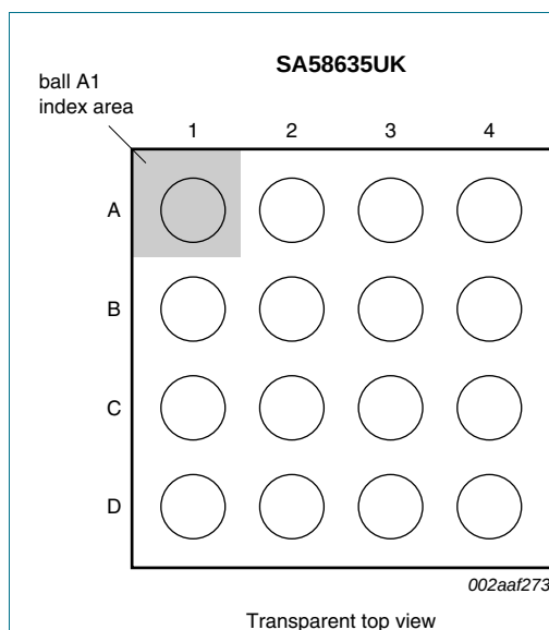
Fig 2. Pin configuration for WLCSP16
