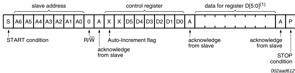
Fig 8. Write to a specific register
