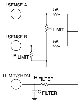
FIGURE B. CURRENT LIMIT WITH SHUTDOWN CURRENT MODE.
