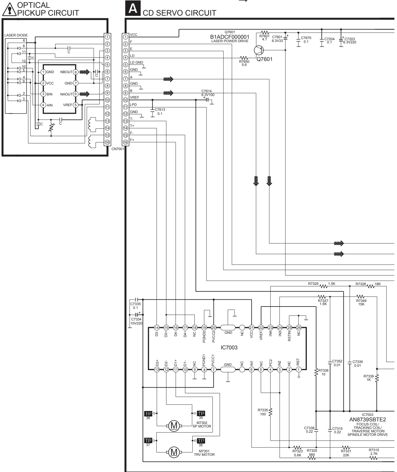
SCHEMATIC DIAGRAM - 1
