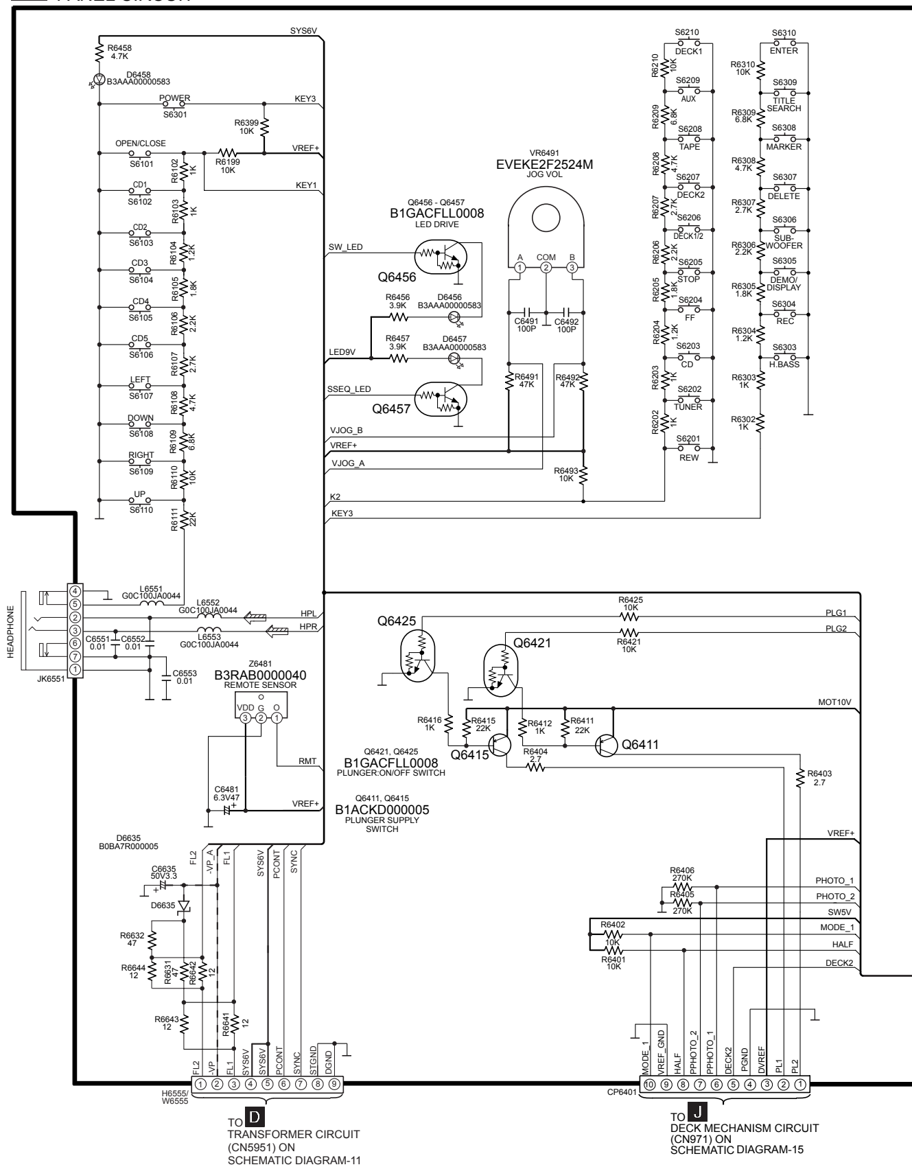
SCHEMATIC DIAGRAM - 9
