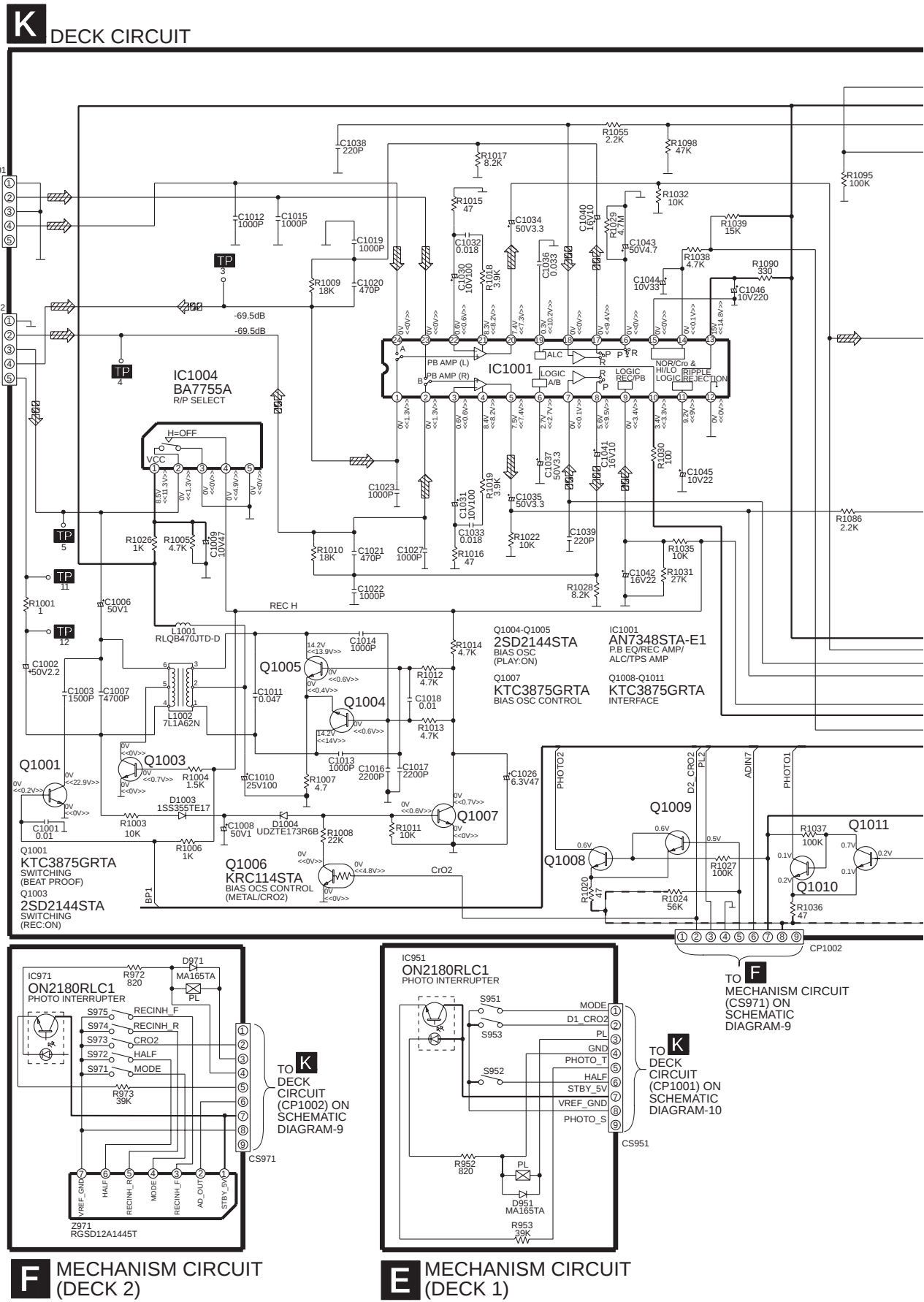
SCHEMATIC DIAGRAM - 9
