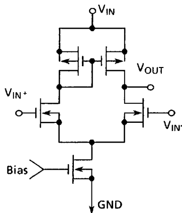
Figure 12 Error amplifier
