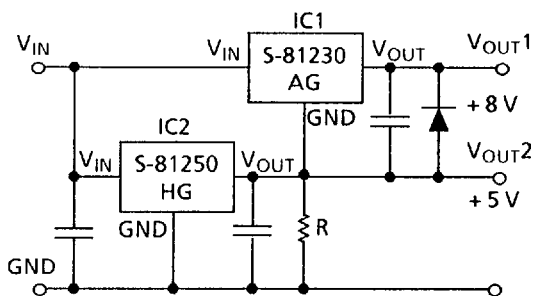
Figure 20 Dual power source
