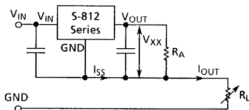
Figure 19 Constant current regulator
