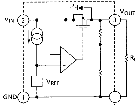
Figure 2 * Parasitic diode
