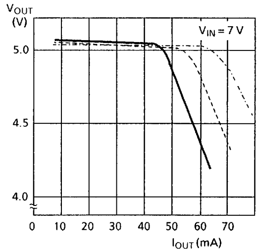
2.6 S-81250HG, S-81250HG-RD-X
