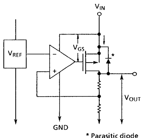
Figure 13 Control transistor
