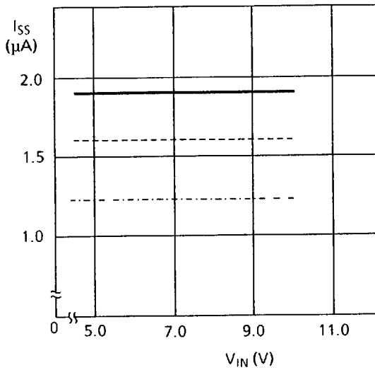
5.5 S-81240AG-RJ-X
