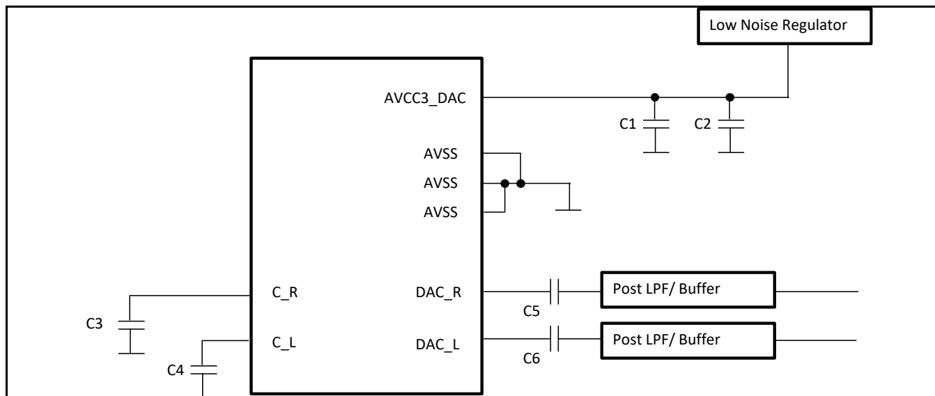
Figure 8-9: Coupling Capacitance (Example)
