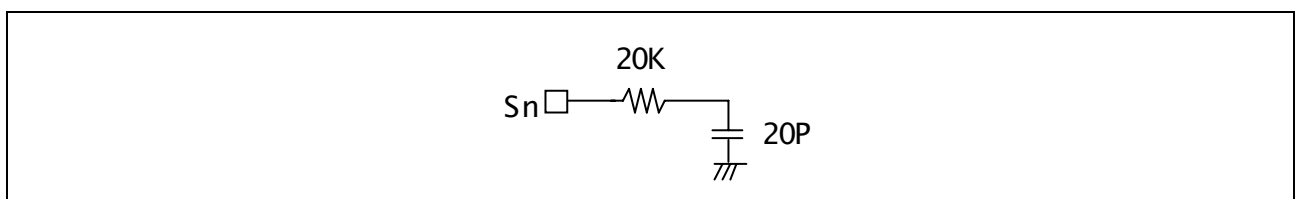
Figure 9. Load condition ( source driver )
