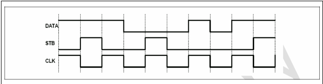
Figure 77. Data-STB encoding
