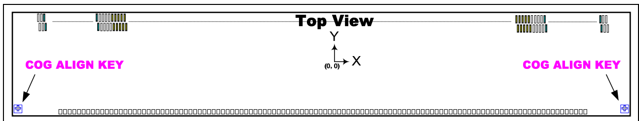
Figure 7. COG align key arrangement layout
