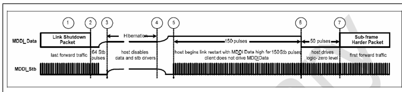
Figure 93. Host-Initiated link wake-up sequence
