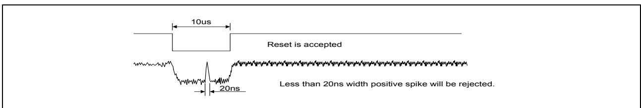
Figure 15. RESX pulse
