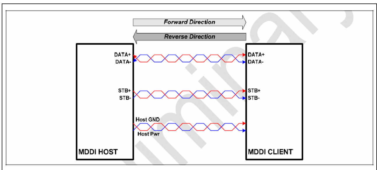
Figure 76. Physical connection of MDDI host and client
