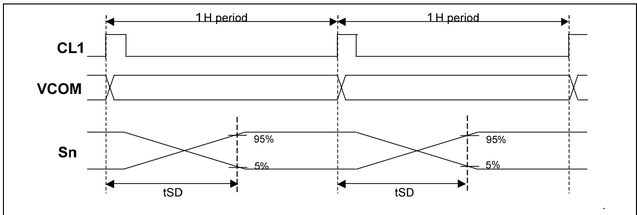
Figure 8. LCD source driver delay
