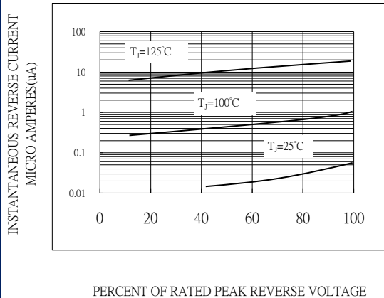
Fig.3-TYPICAL REVERSE CHARACTERISTICS
