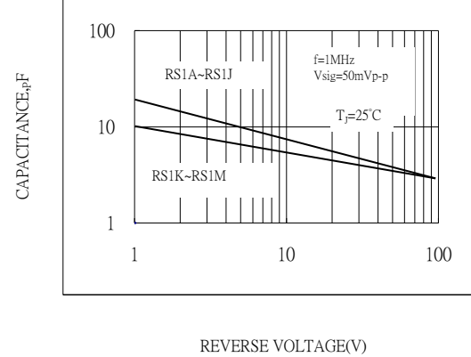
Fig.2-TYPICAL JUNCTION CAPACITANCE
