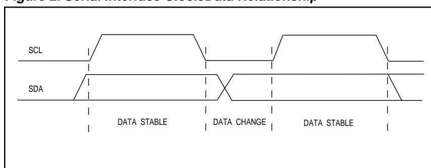
Figure 2. Serial Interface Clock/Data Relationship
