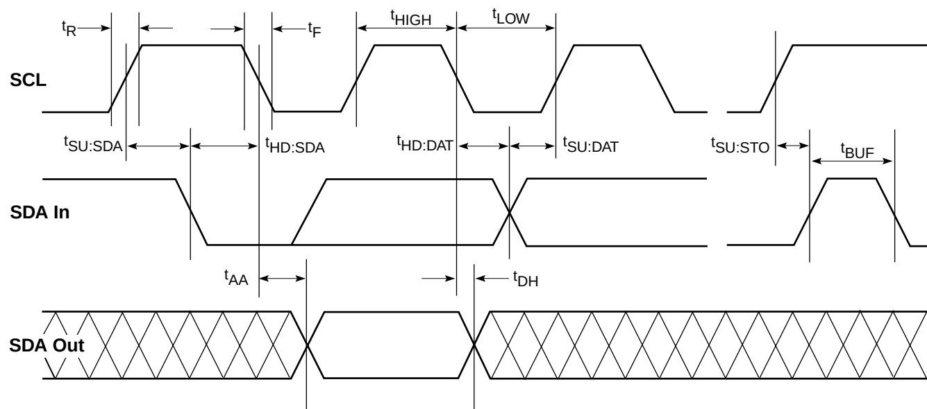
FIGURE 1. BUS TIMING
