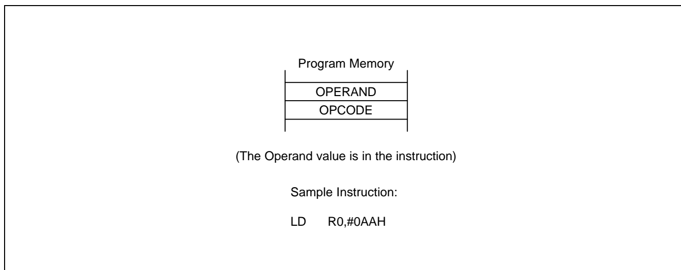
Figure 3-14. Immediate Addressing
