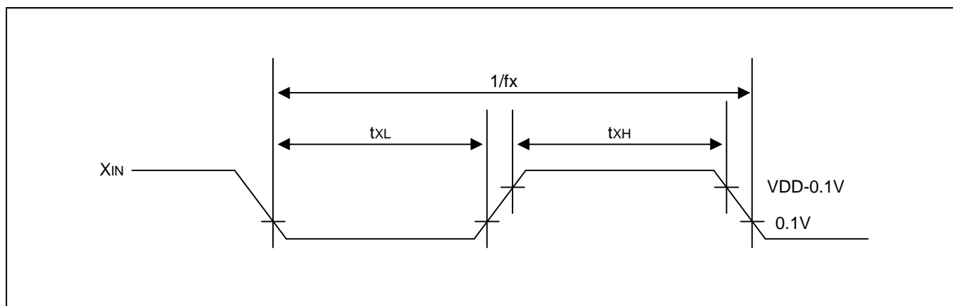
Figure 20-6. Clock Timing Measurement at X_{IN}
