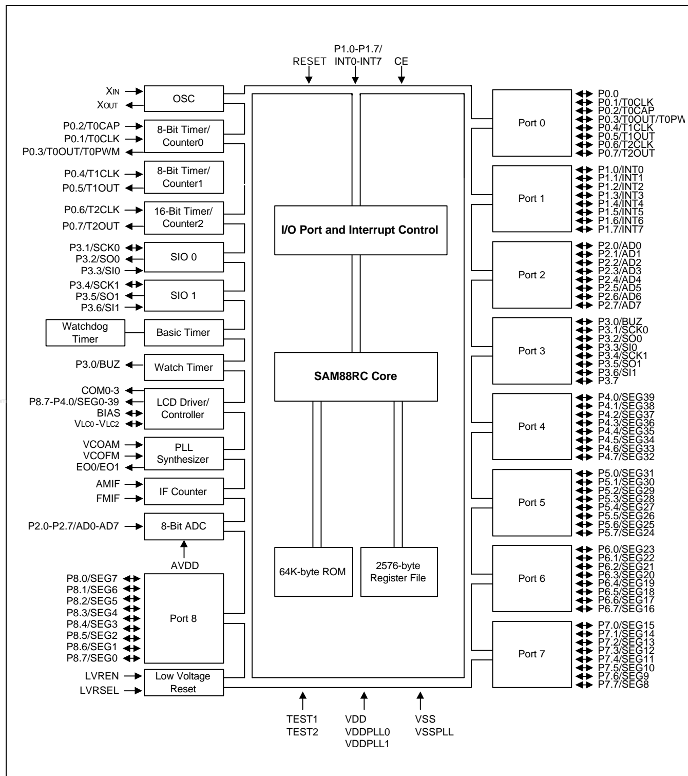
Figure 1-1. Block Diagram
