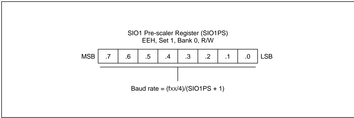
Figure 16-4. SIO1 Pre-scaler Register (SIO1PS)
