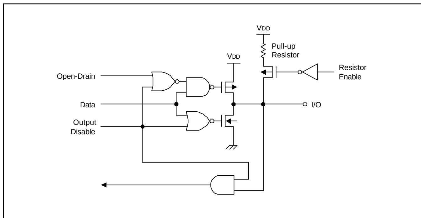
Figure 1-6. Pin Circuit Type E-2 (P5.1-P5.6)
