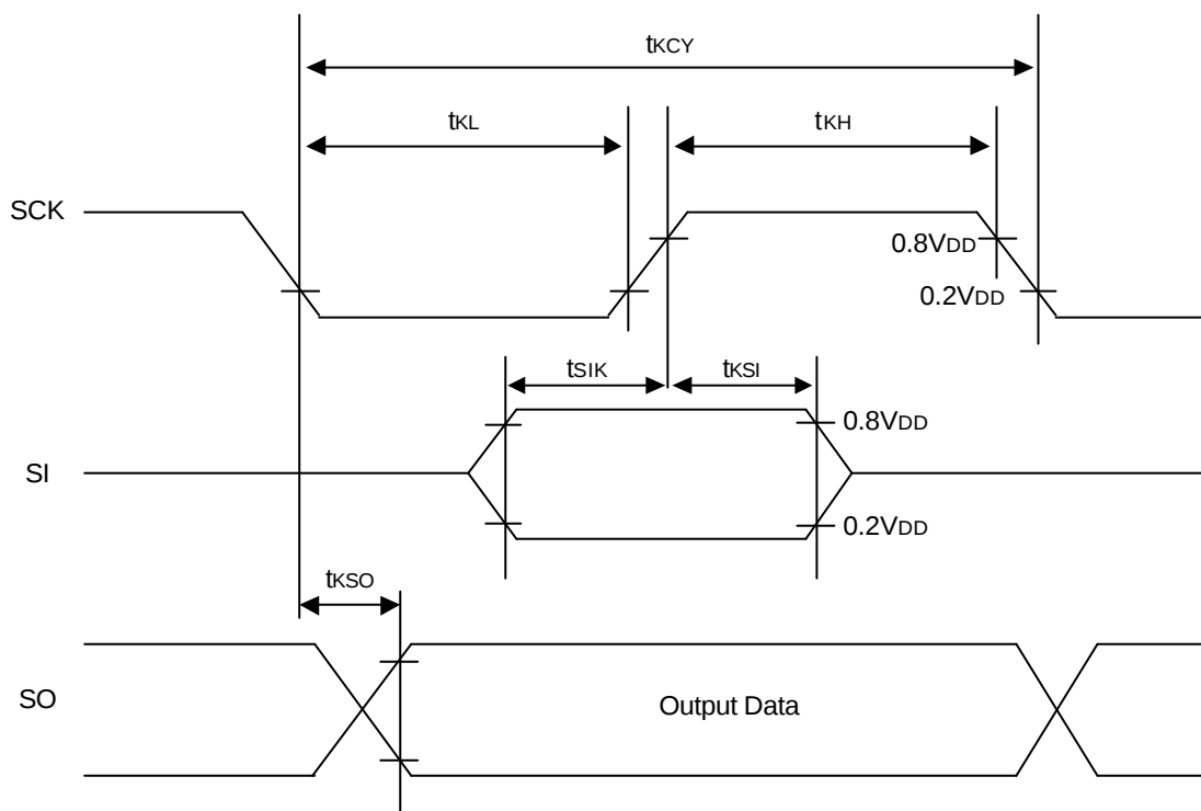
Figure 17-5. Serial Data Transfer Timing
