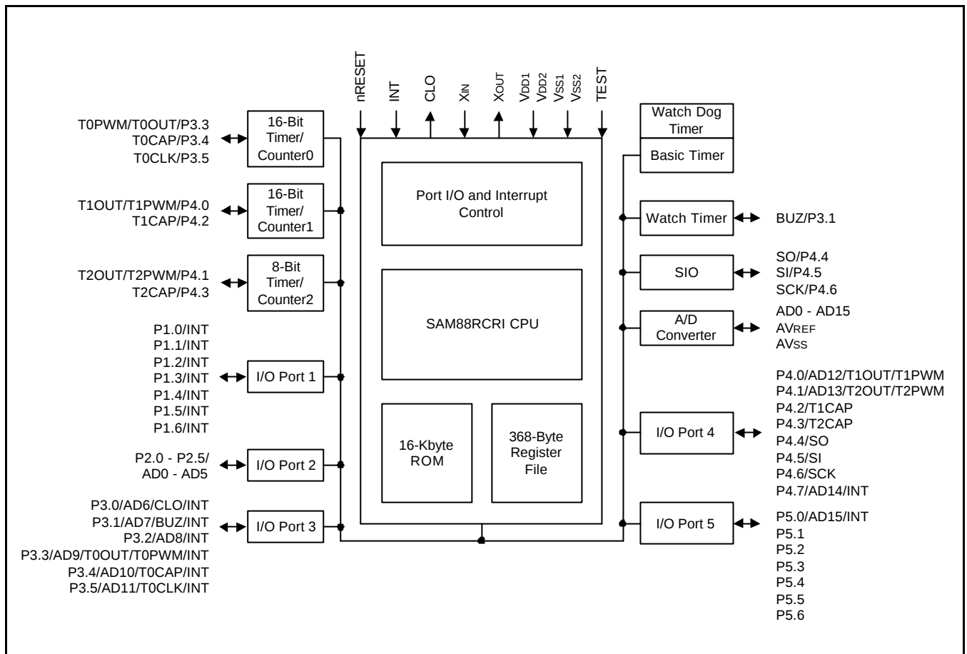
Figure 1-1. Block Diagram
