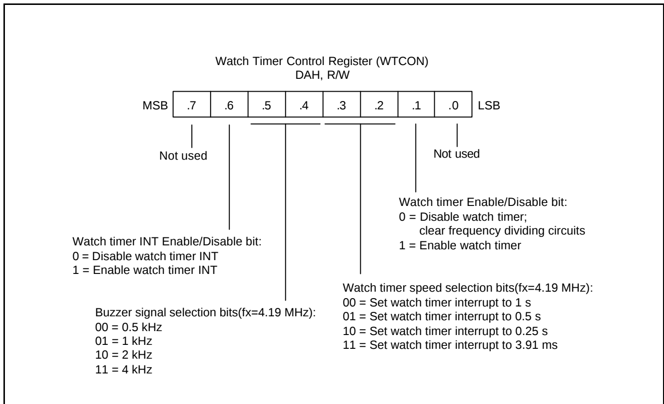
Figure 14-1. Watch Timer Control Register (WTCON)
