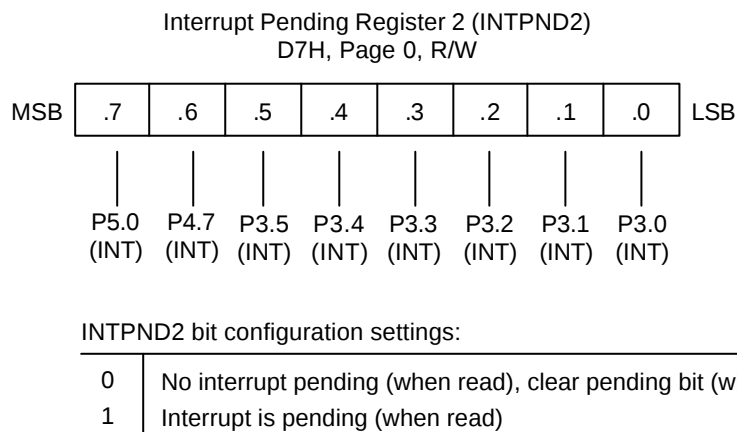
Figure 9-23. Interrupt Pending Register 2 (INTPND2)
