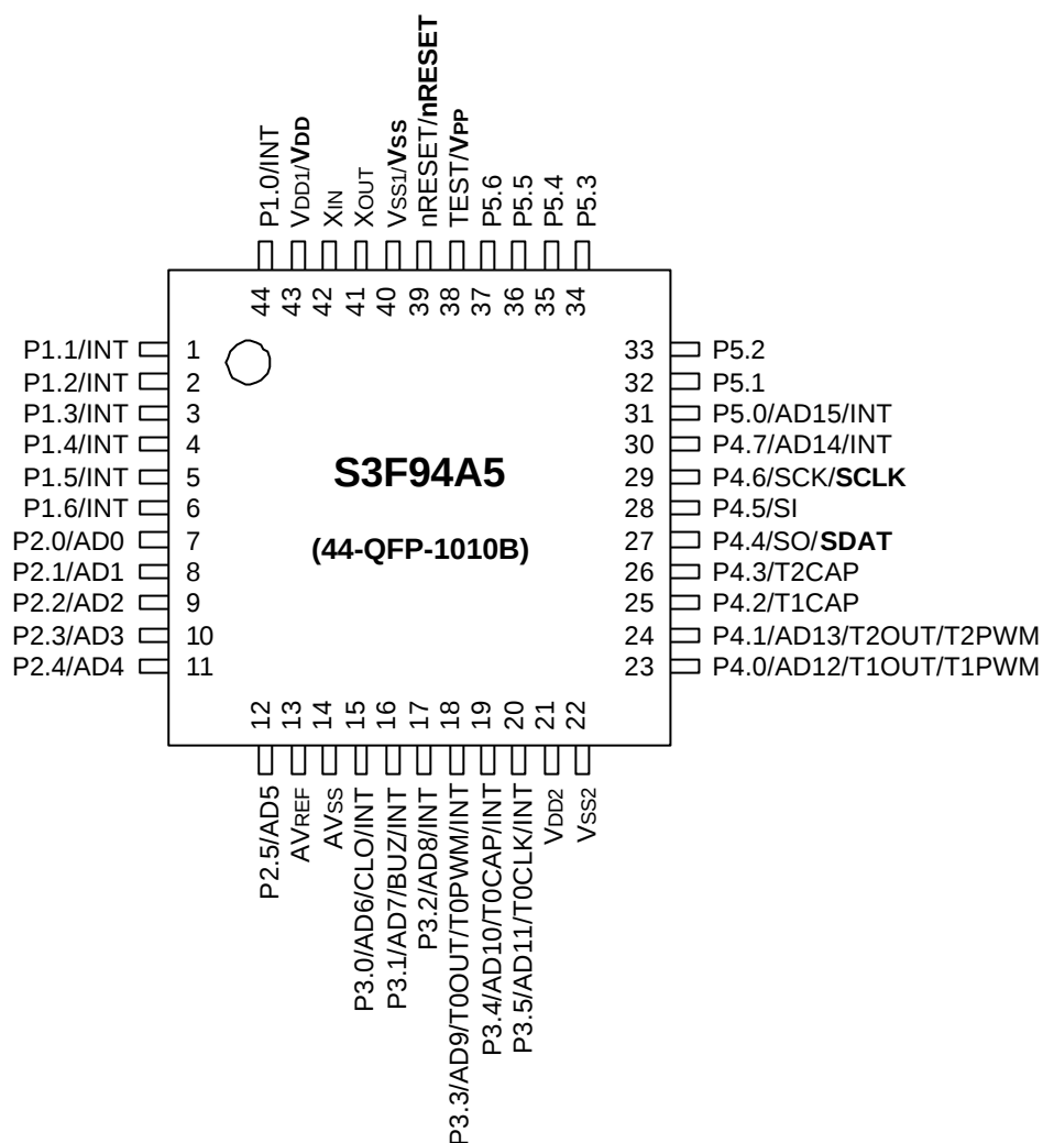
Figure 19-1. S3F94A5 Pin Assignments (44-QFP-1010B)
