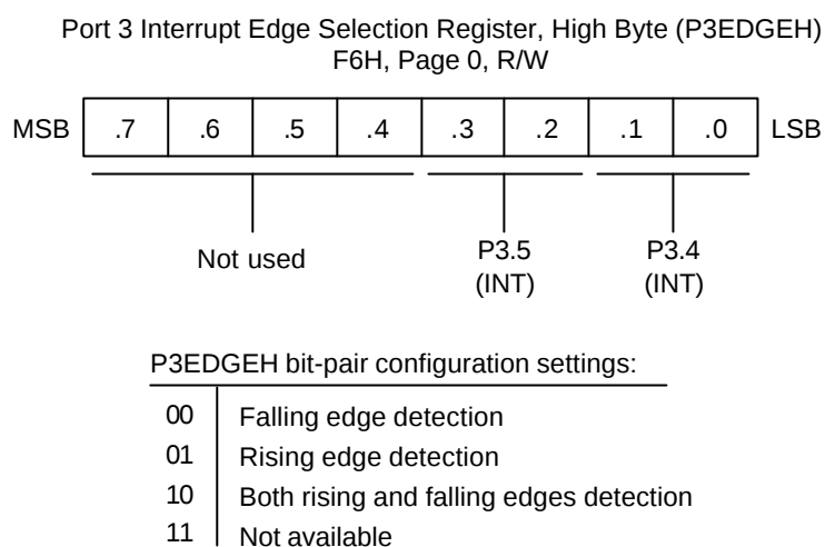
Figure 9-15. Port 3 Interrupt Edge Selection Register, High Byte (P3EDGEH)
