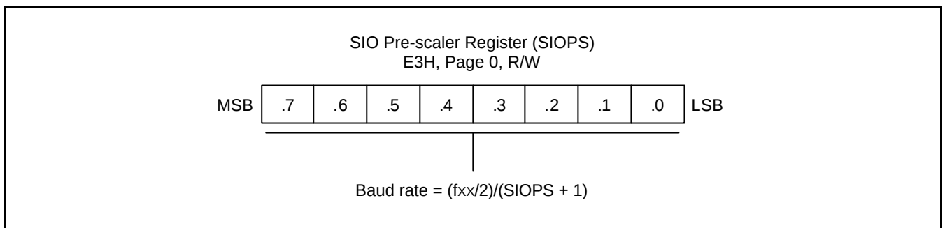
Figure 16-2. SIO Prescaler Register (SIOPS)
