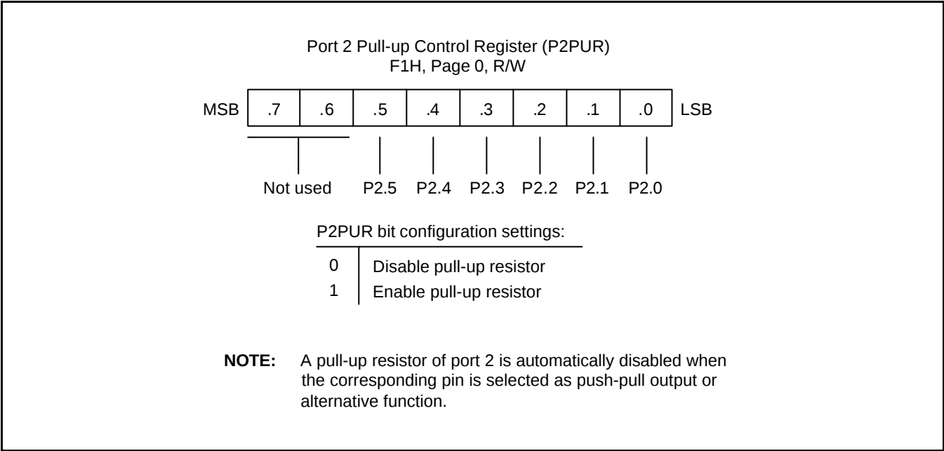
Figure 9-10. Port 2 Pull-up Control Register (P2PUR)
