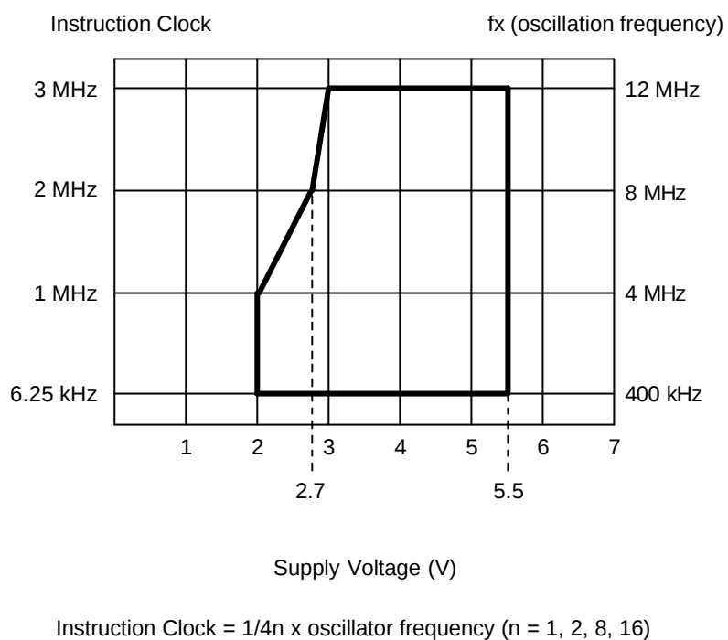
Figure 19-3. Operating Voltage Range
