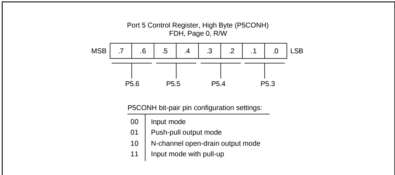
Figure 9-24. Port 5 Control Register, High-Byte (P5CONH)
