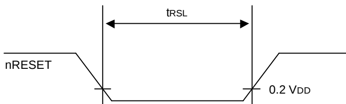
Figure 17-4. Input Timing for nRESET
