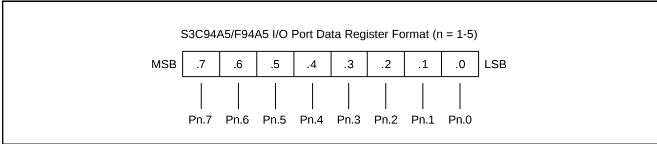
Figure 9-1. S3C94A5/F94A5 I/O Port Data Register Format
