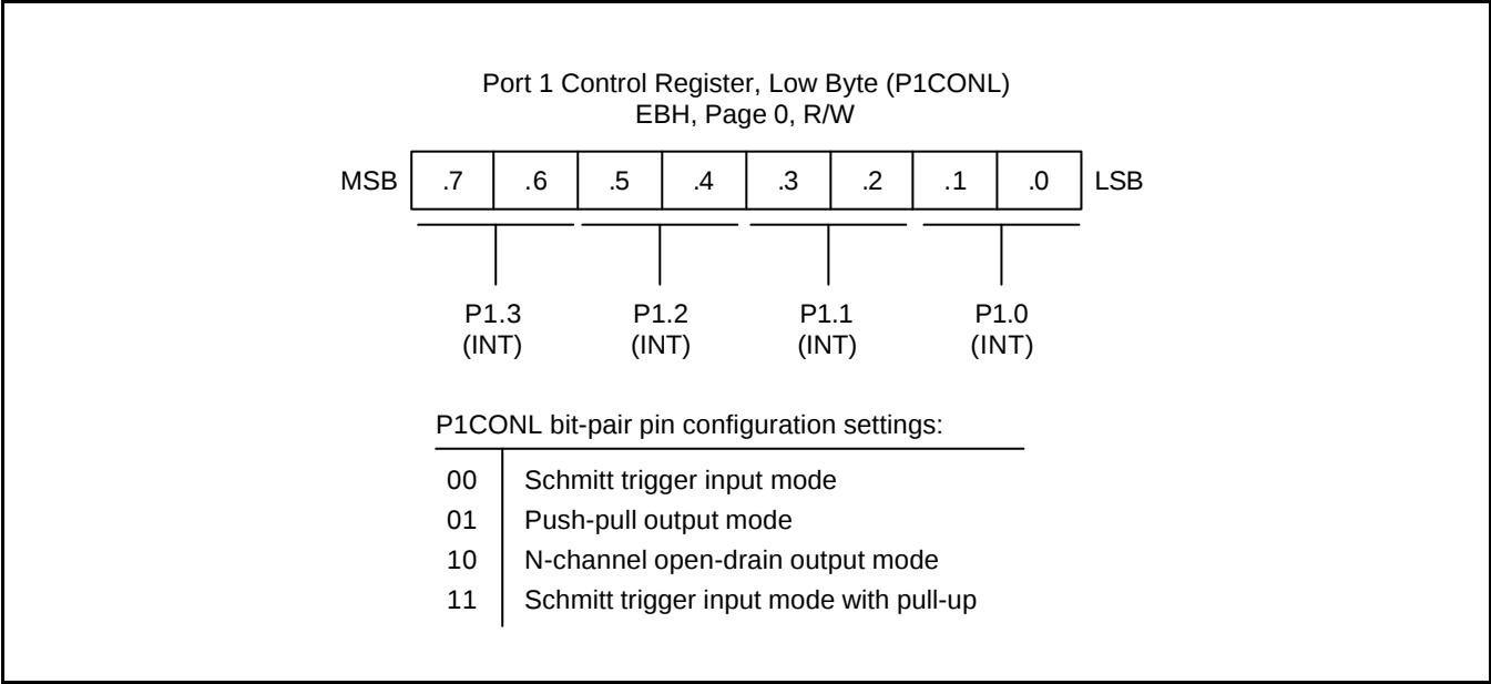
Figure 9-3. Port 1 Control Register, Low Byte (P1CONL)
