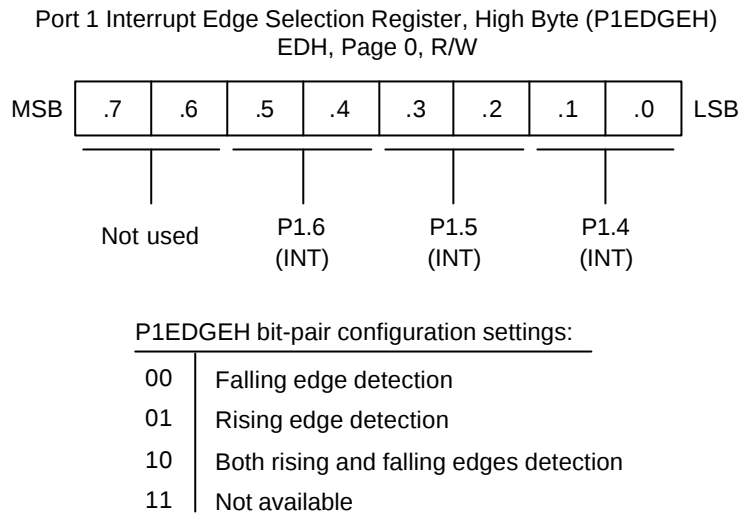
Figure 9-6. Port 1 Interrupt Edge Selection Register, High Byte (P1EDGEH)
