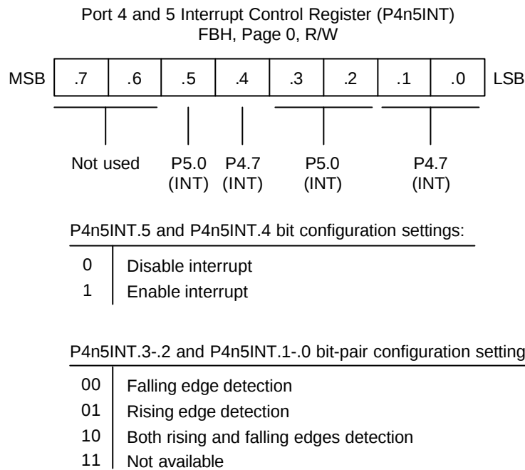
Figure 9-22. Port 4 and 5 Interrupt Control Register (P4n5INT)
