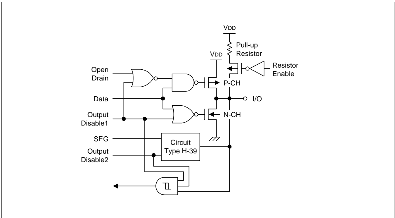
Figure 1-17. Pin Circuit Type H-41 (P6-P8)
