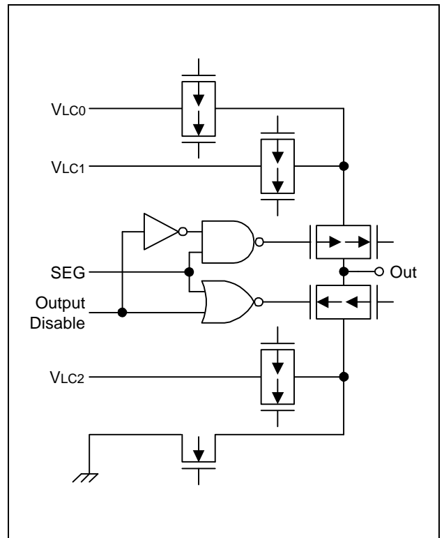
Figure 1-16. Pin Circuit Type H-39
