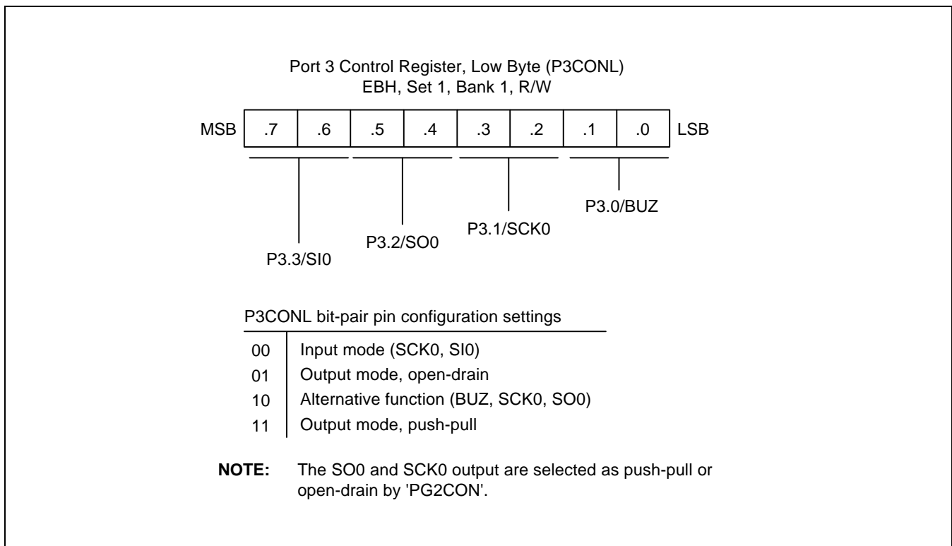
Figure 9-11. Port 3 Low-Byte Control Register (P3CONL)
