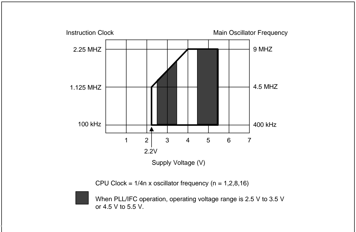
Figure 22-3. Operating Voltage Range
