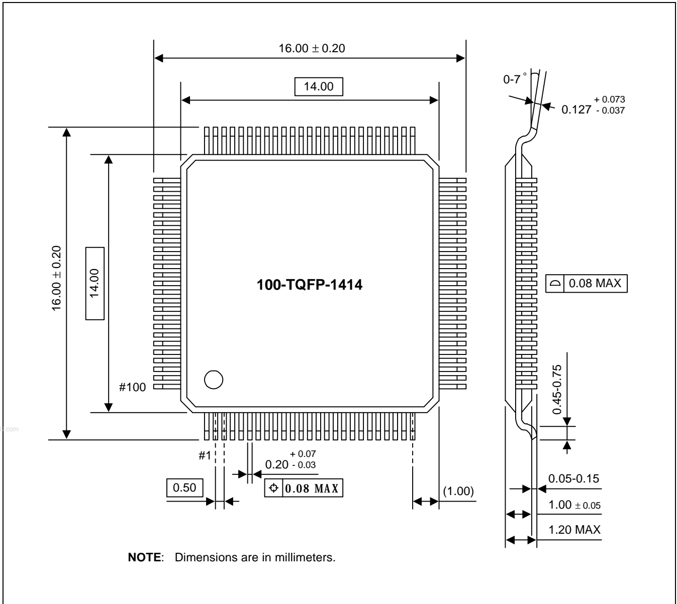
Figure 21-2. Package Dimensions (100-TQFP-1414)
