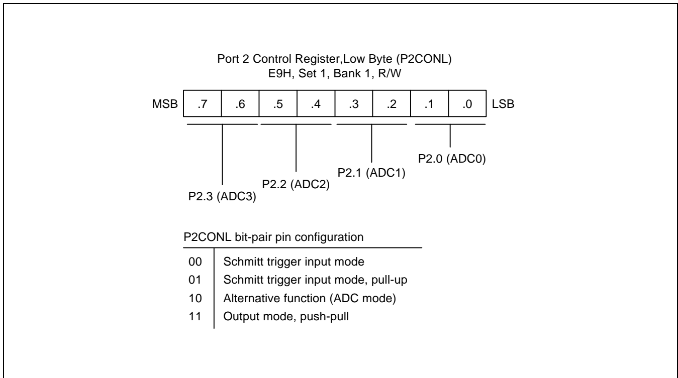
Figure 9-9. Port 2 Low-Byte Control Register (P2CONL)
