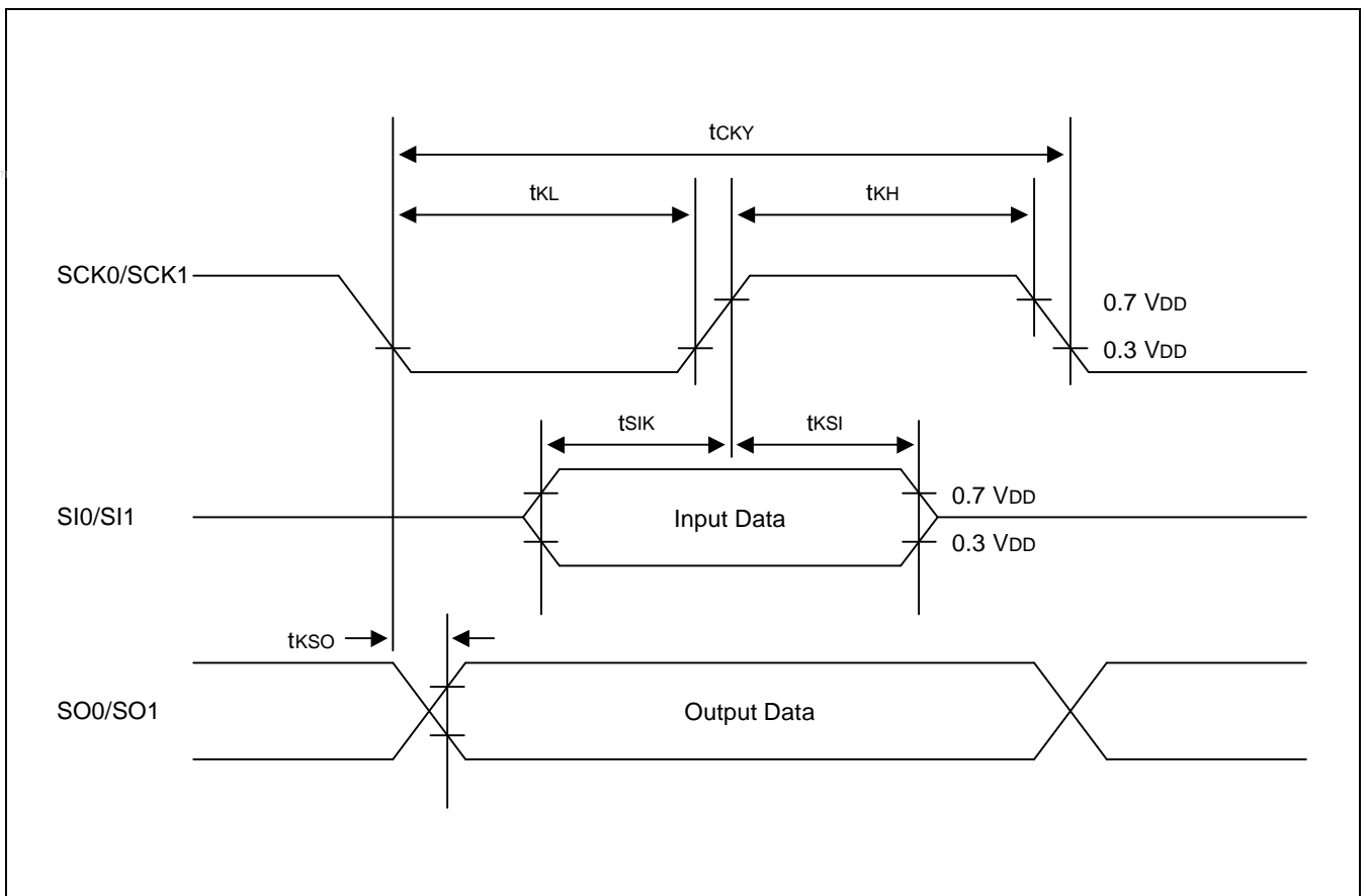
Figure 20-5. Serial Data Transfer Timing
