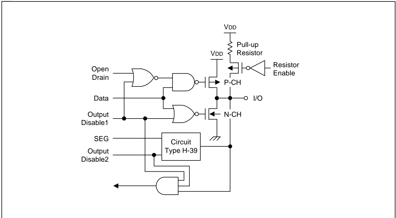
Figure 1-18. Pin Circuit Type H-42 (P4, P5)
