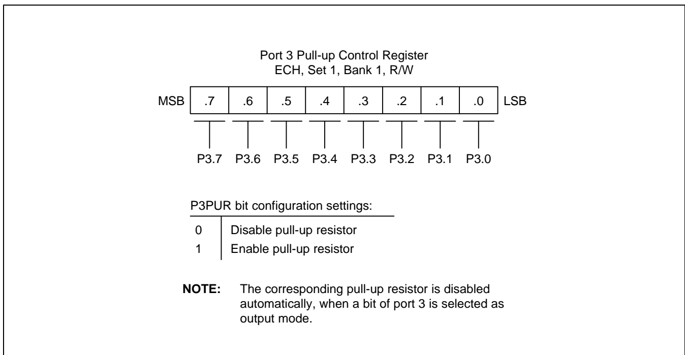
Figure 9-12. Port 3 Pull-up Control Register (P3PUR)
