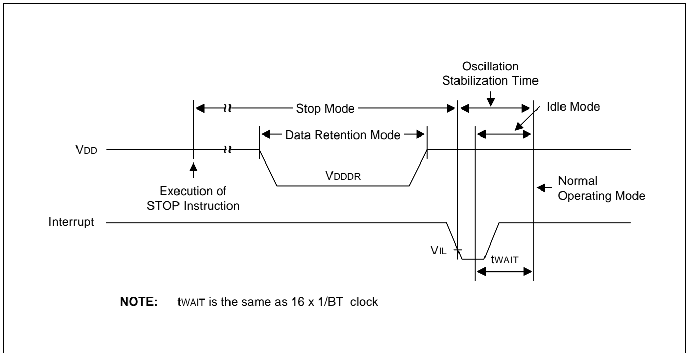
Figure 20-4. Stop Mode Release Timing Initiated by Interrupts
