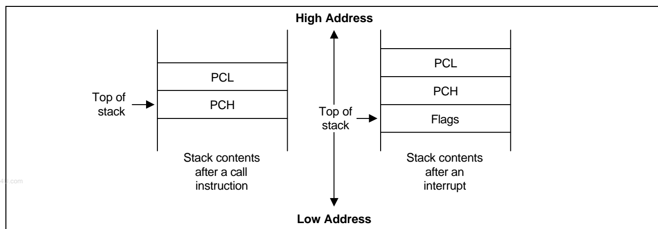
Figure 2-15. Stack Operations
