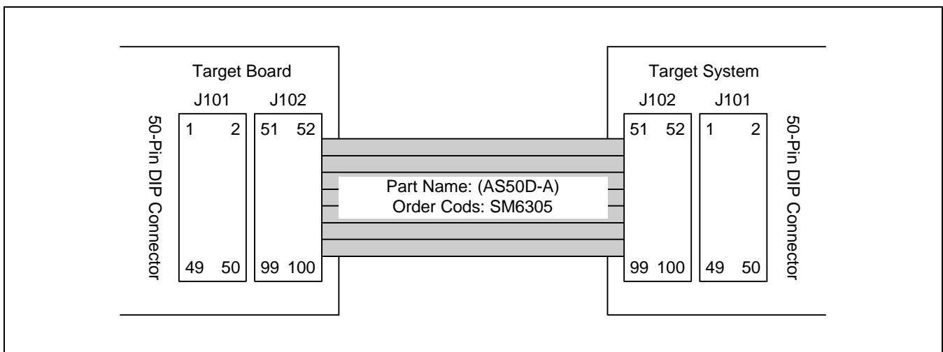
Figure 23-4. S3C831B/P831B Probe Adapter Cables for 100-QFP Package
