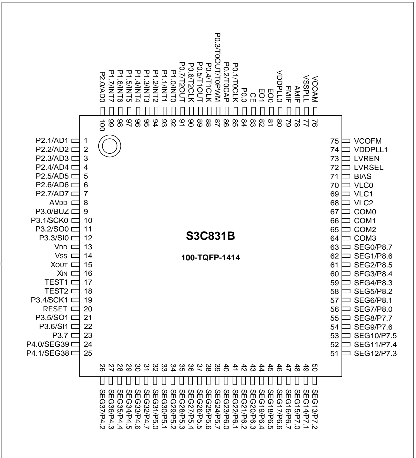
Figure 1-3. S3C831B Pin Assignments (100-TQFP-1414)
