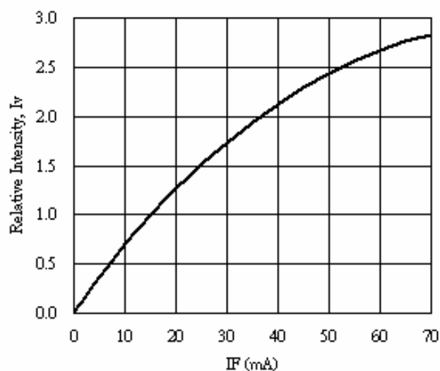
Forward Current vs. Relative Luminosity (Ta=25°C)
