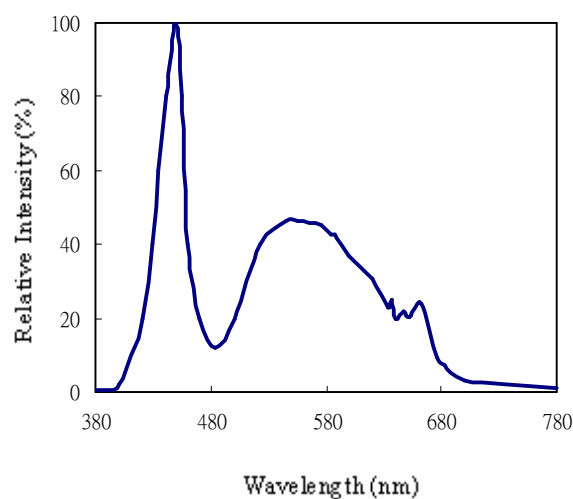
* Spectrum (Ta=25°C)
