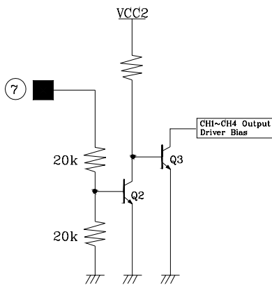
Fig2. Mute function
