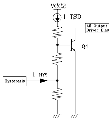
Fig3.Thermal shut down
