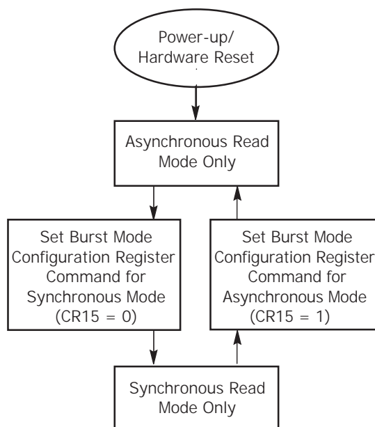
Figure 7.I. Synchronous/Asynchronous State Diagram
