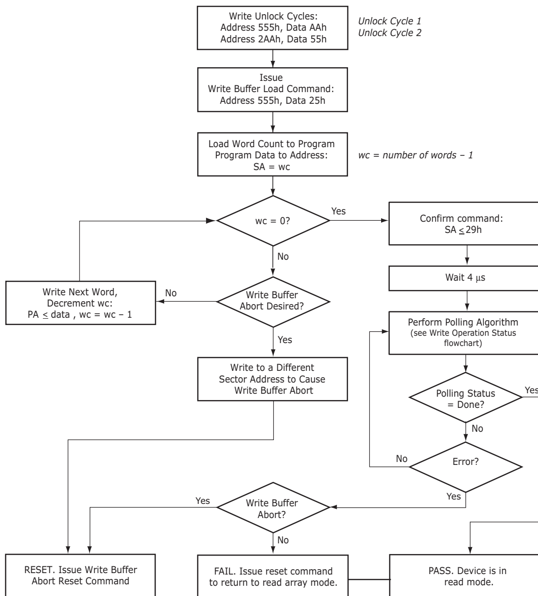
Figure 7.2 Write Buffer Programming Operation
