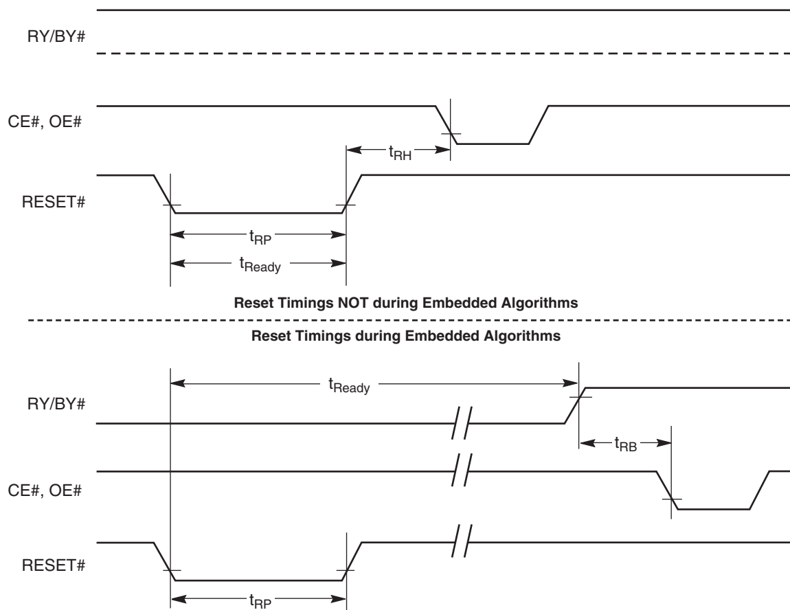
Figure 20.5 Reset Timings
