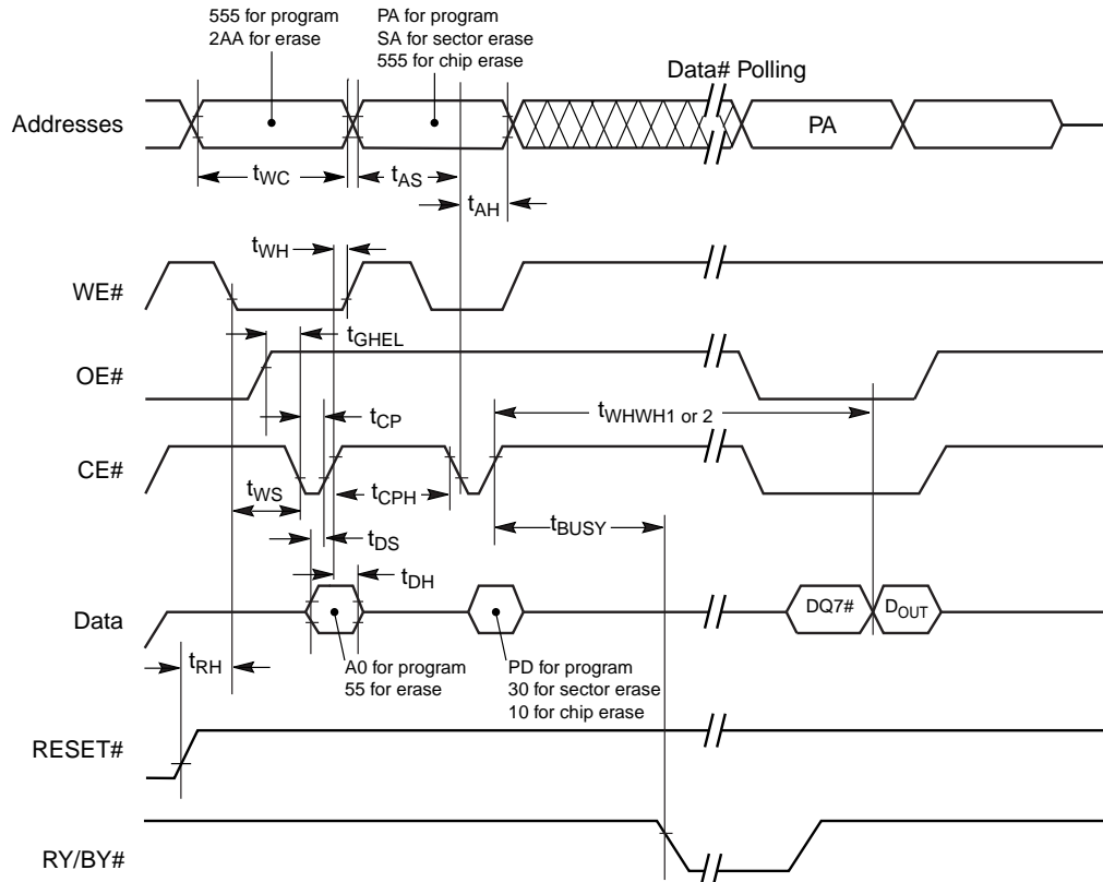
Figure 18.12 Alternate CE# Controlled Write Operation Timings
