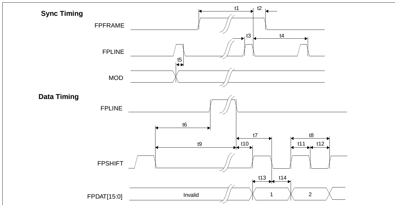
Figure 6-31: Dual Color 16-Bit Panel A.C. Timing
