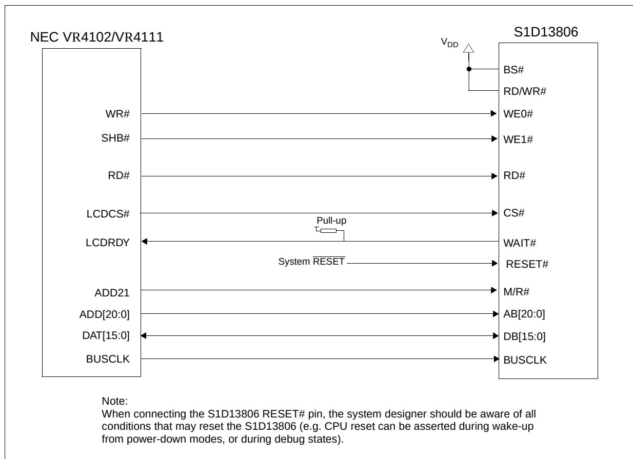
Figure 4-1: Typical Implementation of NEC VR4102/VR4111 to S1D13806 Interface
