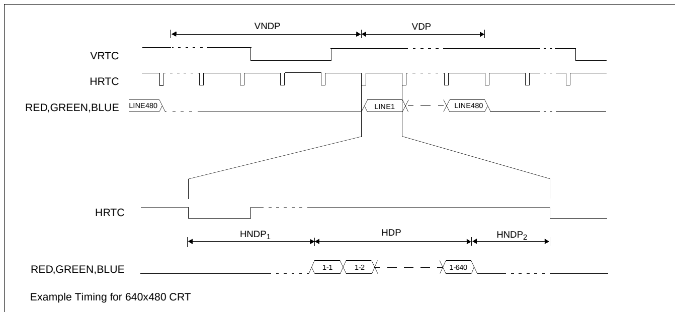
Figure 6-34: CRT Timing
