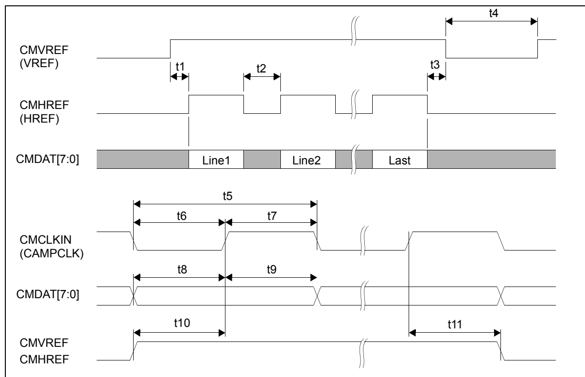
Figure 7-41: Camera Interface Timing
