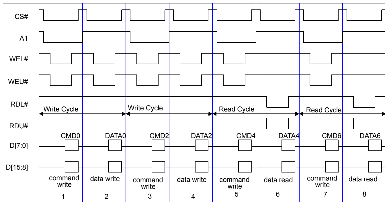
Figure 22-1: Register Read/Write" Example Sequence
