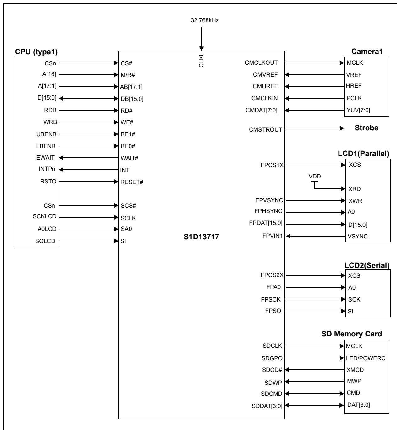
Figure 3-3: S1D13717 System Diagram 3
