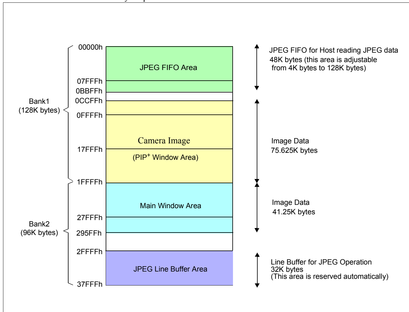
Figure 8-10: Memory Map for Main Window, PIP + Window, Overlay and JPEG
