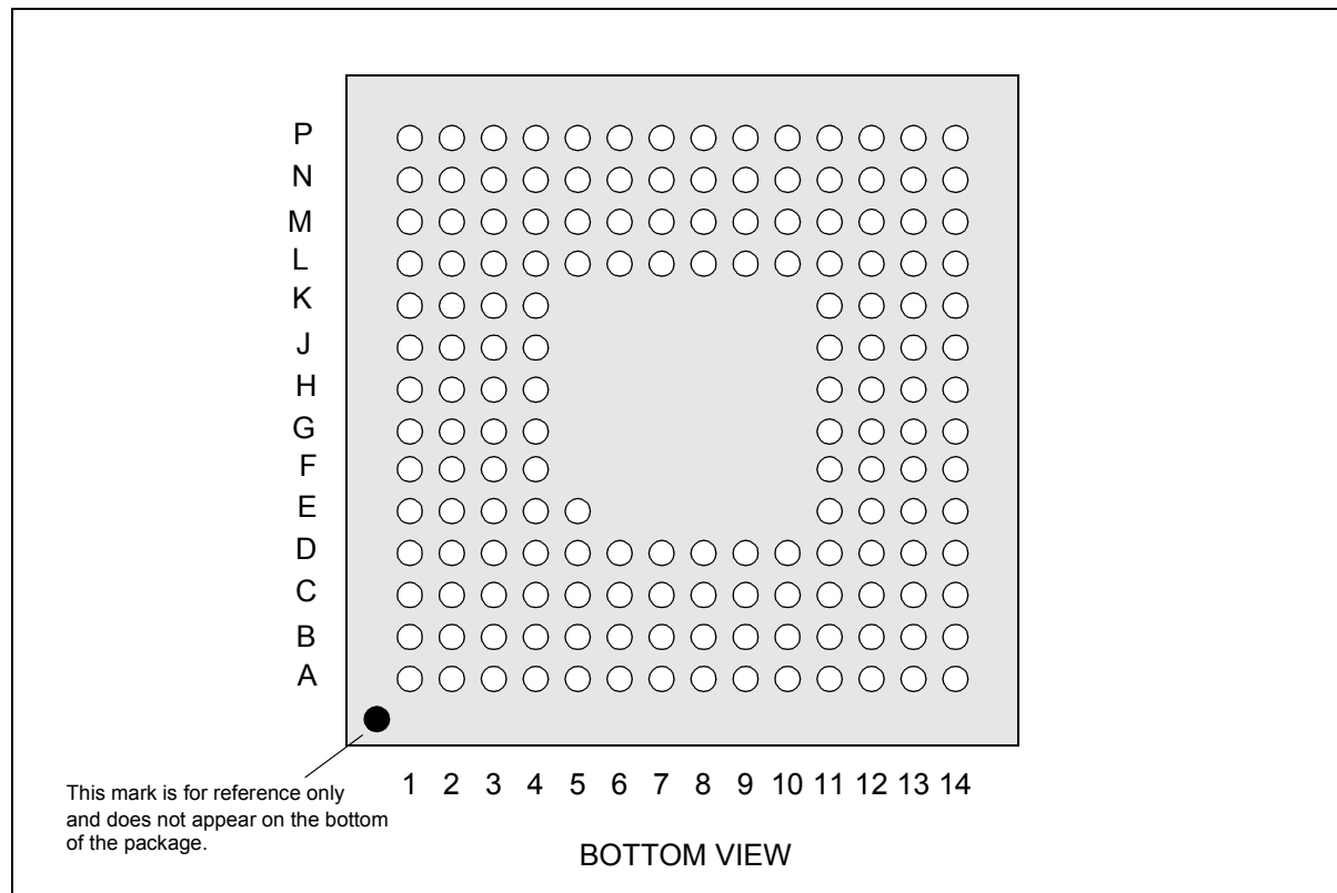
Figure 5-1: S1D13717 FCBGA-161 Pin Mapping
