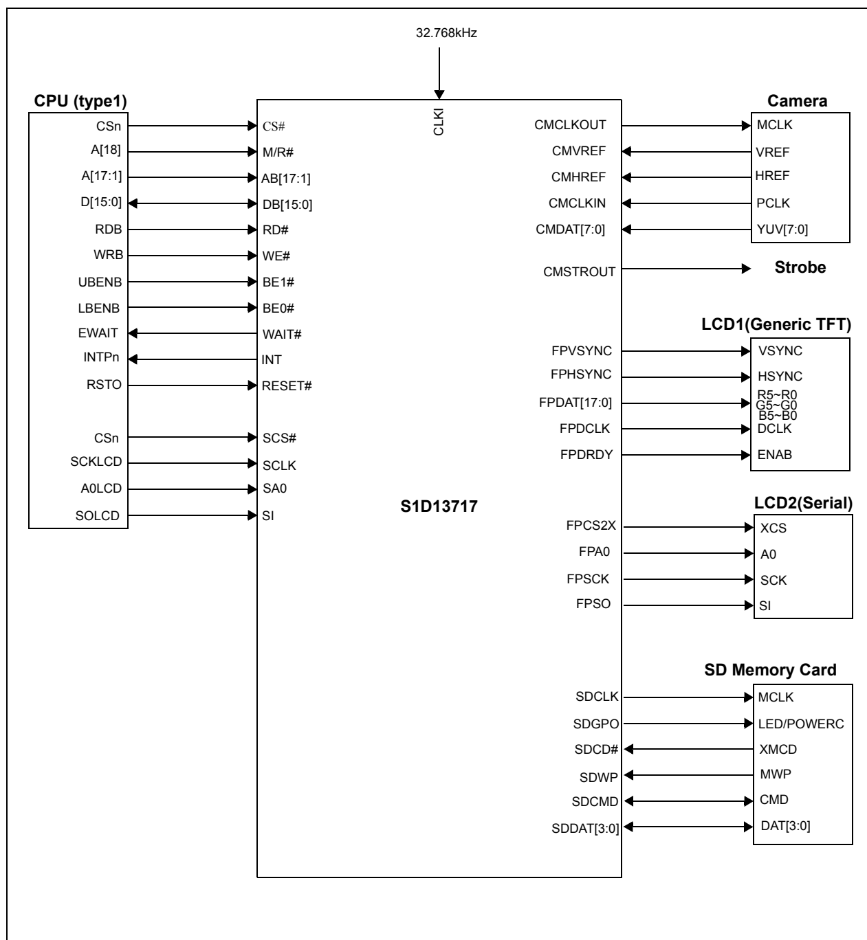
Figure 3-1: S1D13717 System Diagram 1
