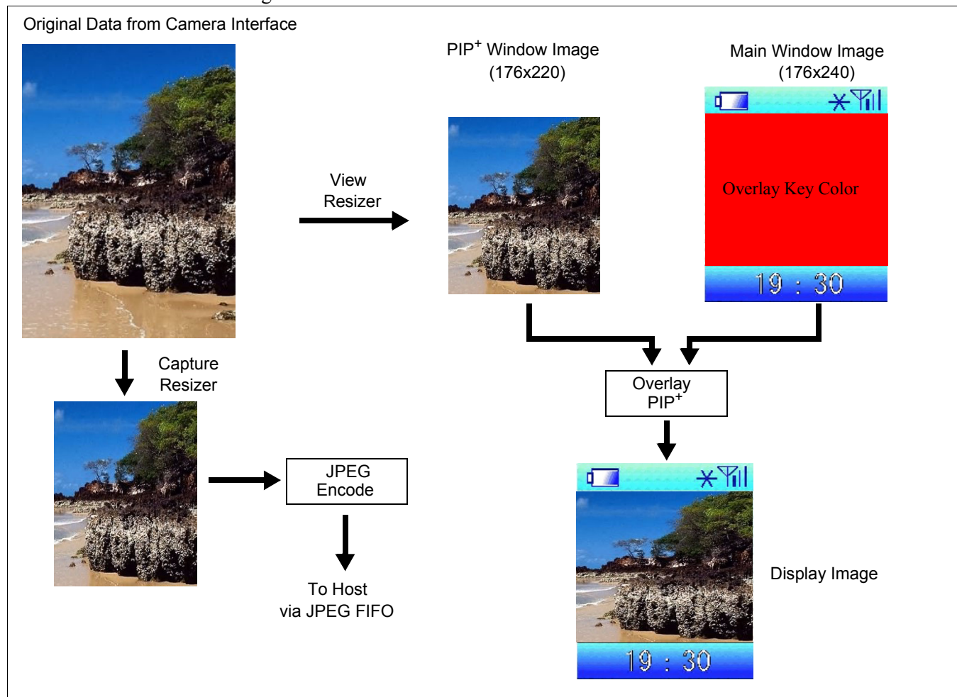
Figure 8-9: Main Window, PIP + Window, Overlay, and JPEG
