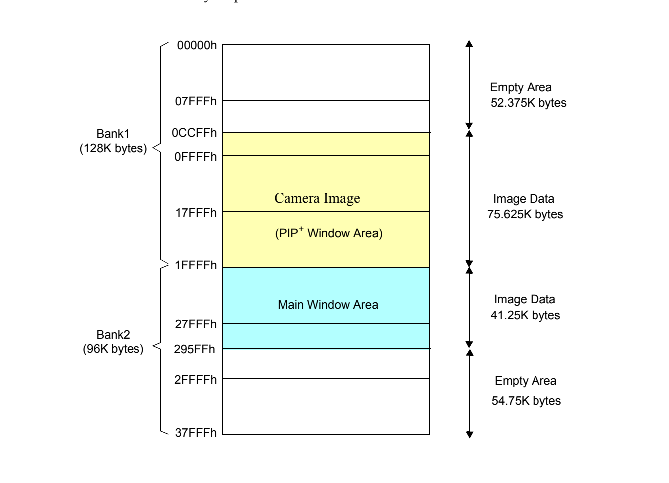
Figure 8-8: Memory Map for Main Window, PIP + Window, Overlay, and YUV
