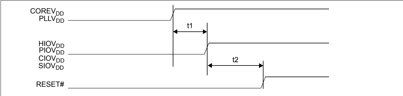
Figure 7-4: Power-On Sequence
