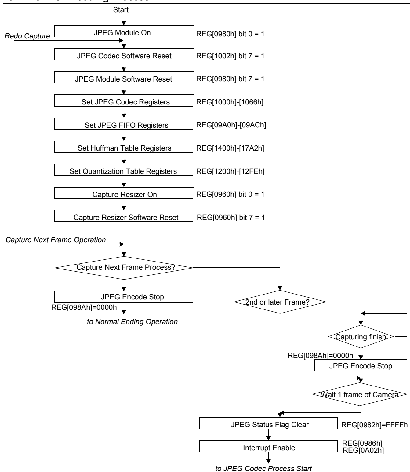
Figure 19-2: JPEG Encoding Process (1 of 4)
