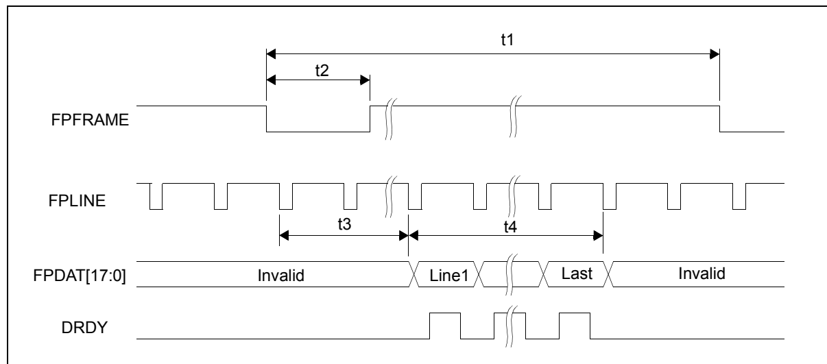
Figure 7-32: Generic RGB Type Interface Panel Vertical timing
