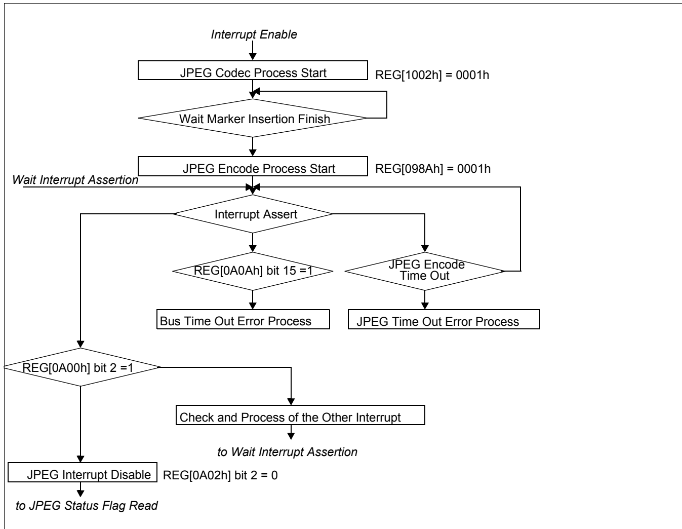
Figure 19-3: JPEG Encoding Process (2 of 4)
