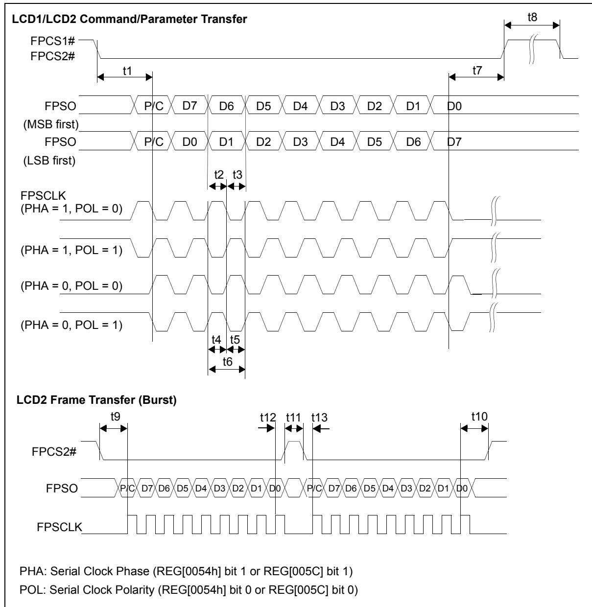
Figure 7-34: LCD1 ND-TFD, LCD2 9-Bit Serial Interface Timing
