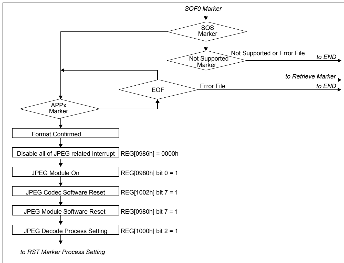
Figure 19-7: JPEG Decoding Process (2 of 6)
