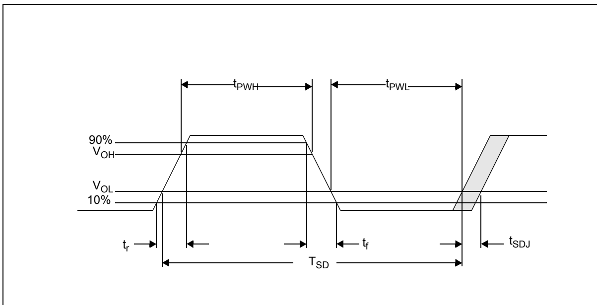
Figure 7-45: SD Memory Card Clock Output Timing
