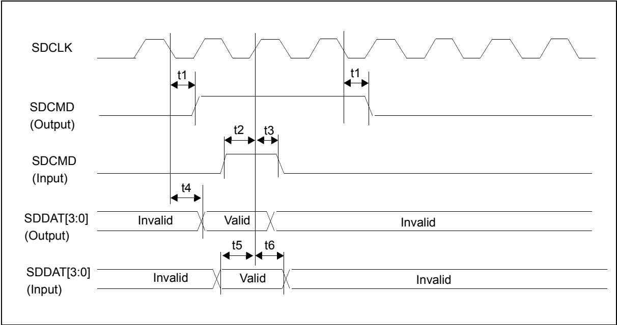
Figure 7-44: SD Memory Card Access Timing
