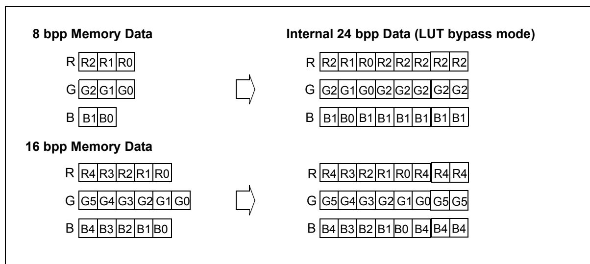
Figure 13-7: Data Bit Cover When the LUT is Bypassed
