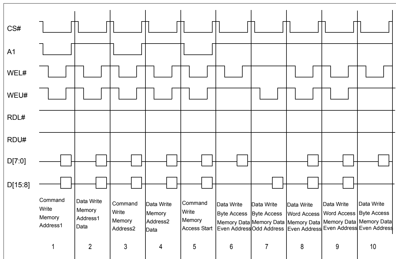
Figure 22-2: Memory Write Example Sequence
