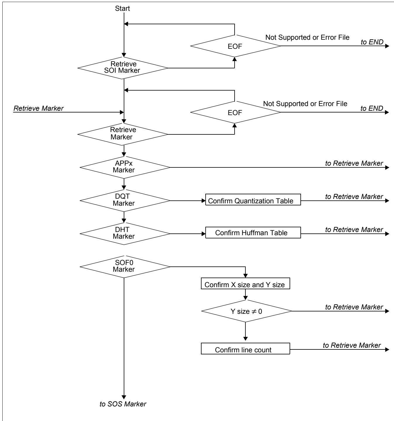
Figure 19-6: JPEG Decoding Process (1 of 6)
