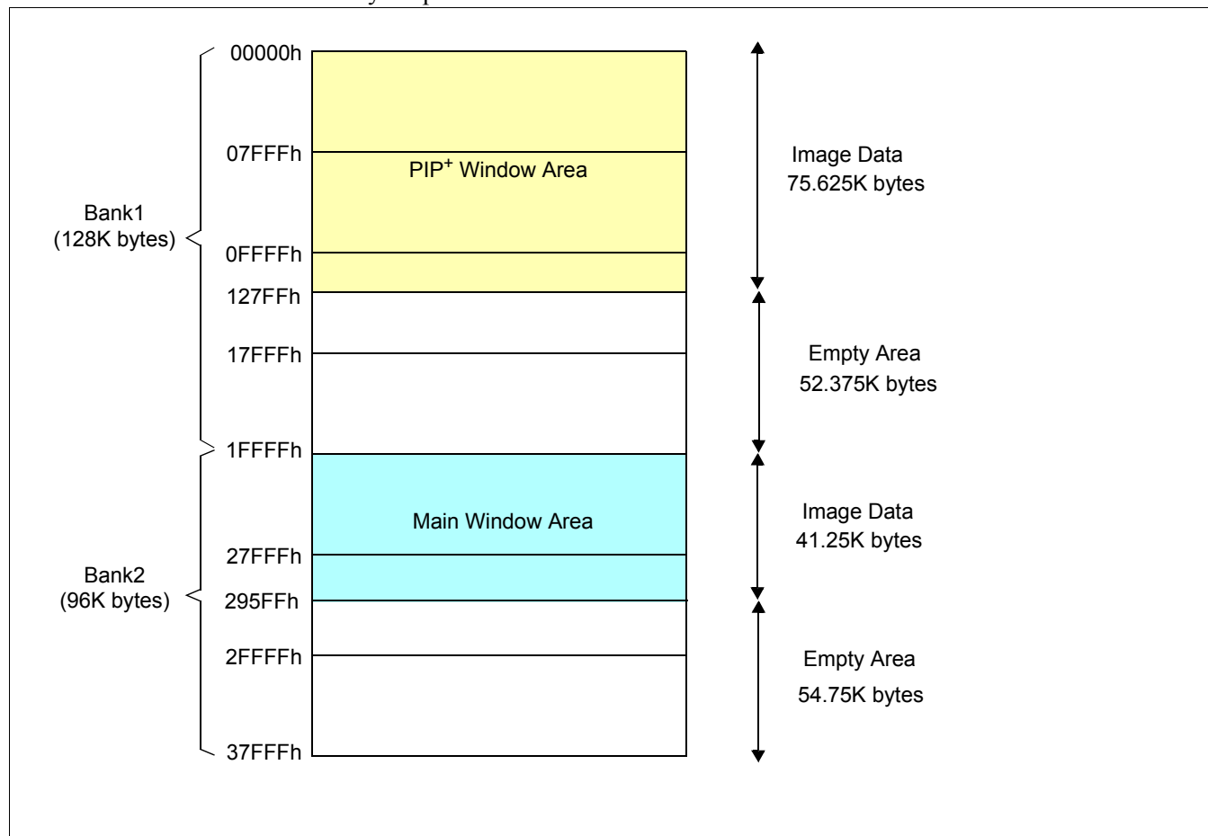
Figure 8-6: Memory Map for Main Window, PIP+ Window, and Overlay Display
