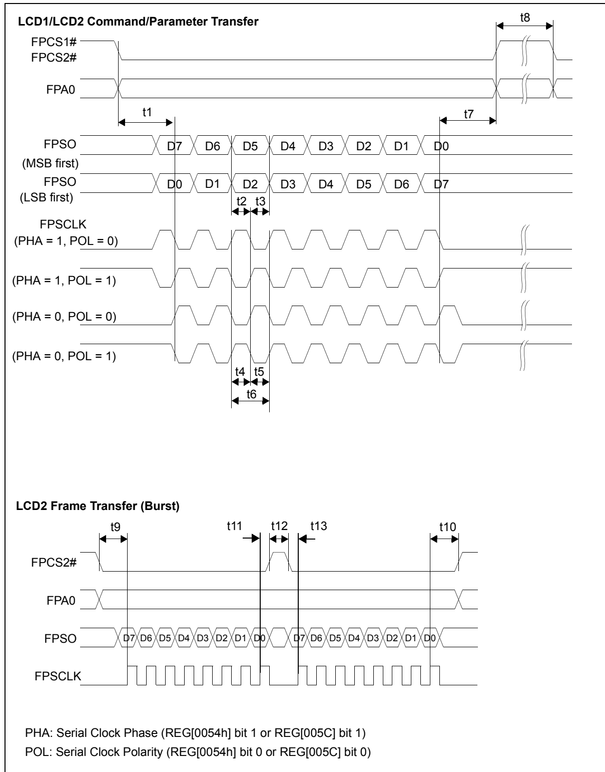
Figure 7-33: LCD1 ND-TFD, LCD2 8-Bit Serial Interface Timing
