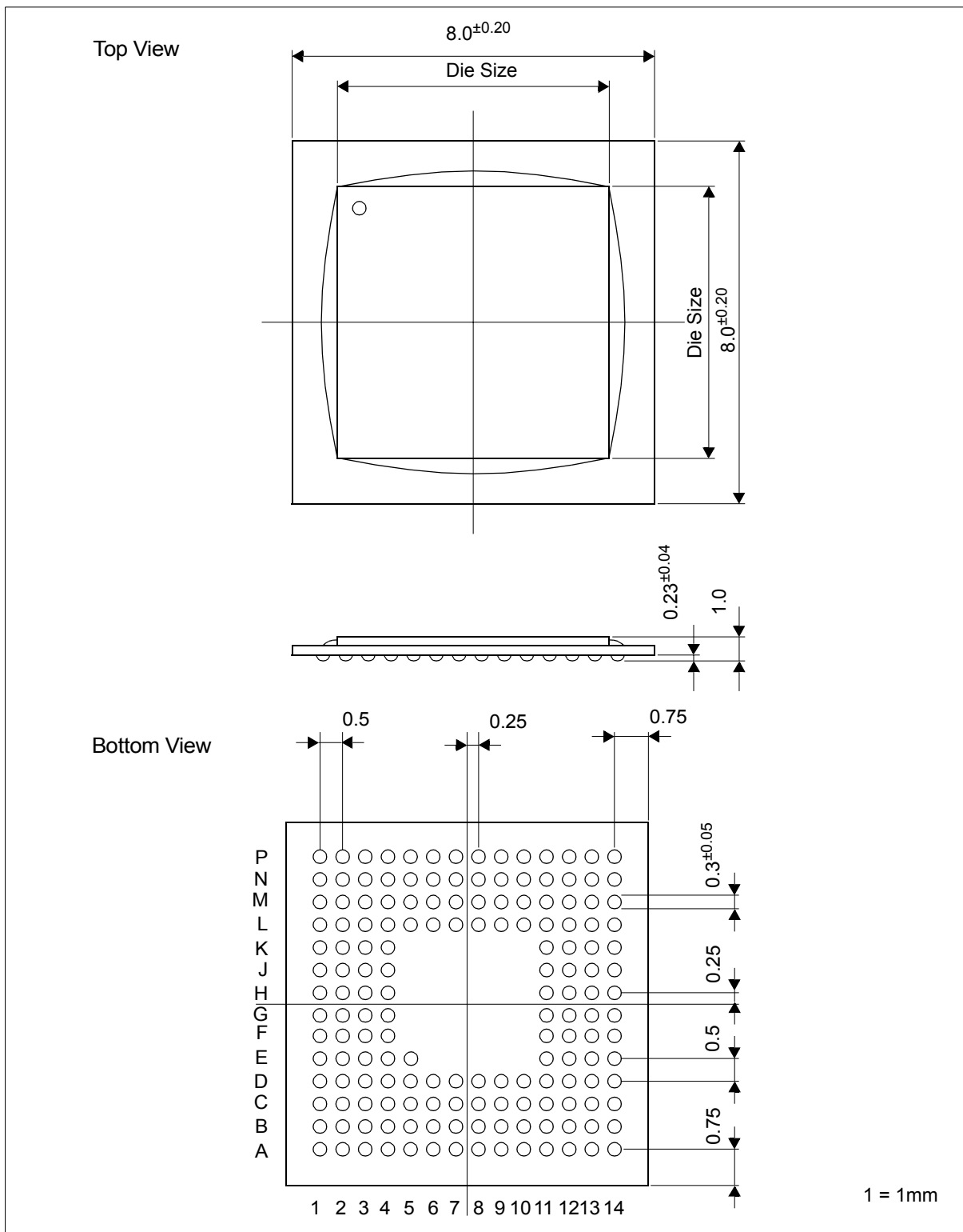
Figure 23-1: S1D13717 FCBGA-161 Pin Package
