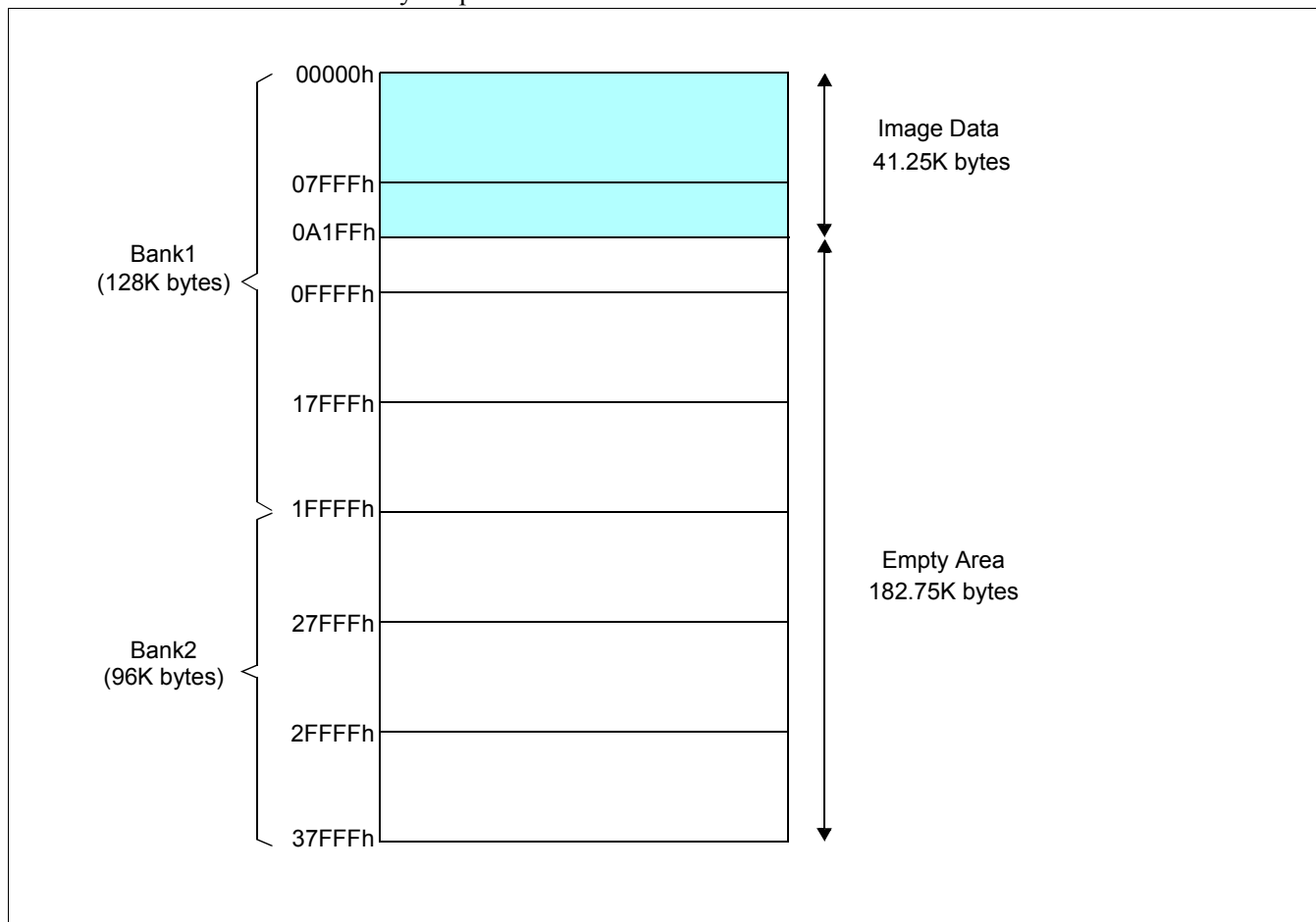
Figure 8-2: Memory Map for Main Window Case 1
