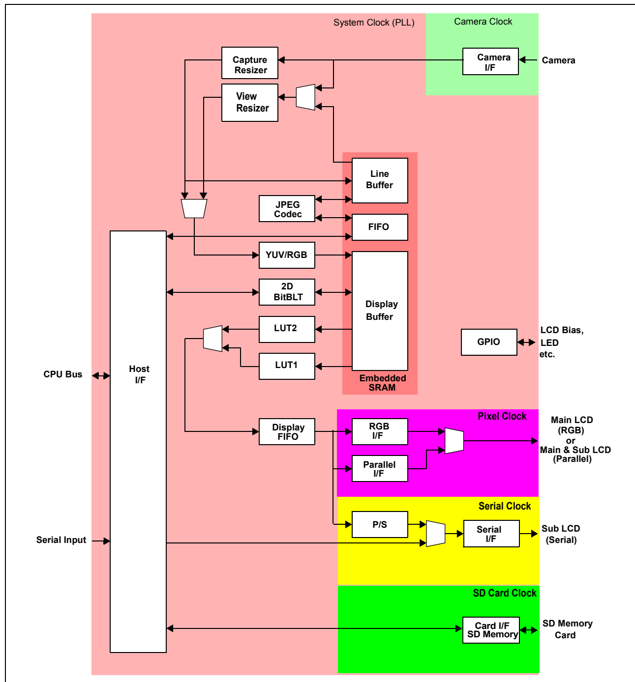
Figure 4-1: S1D13717 Block Diagram
