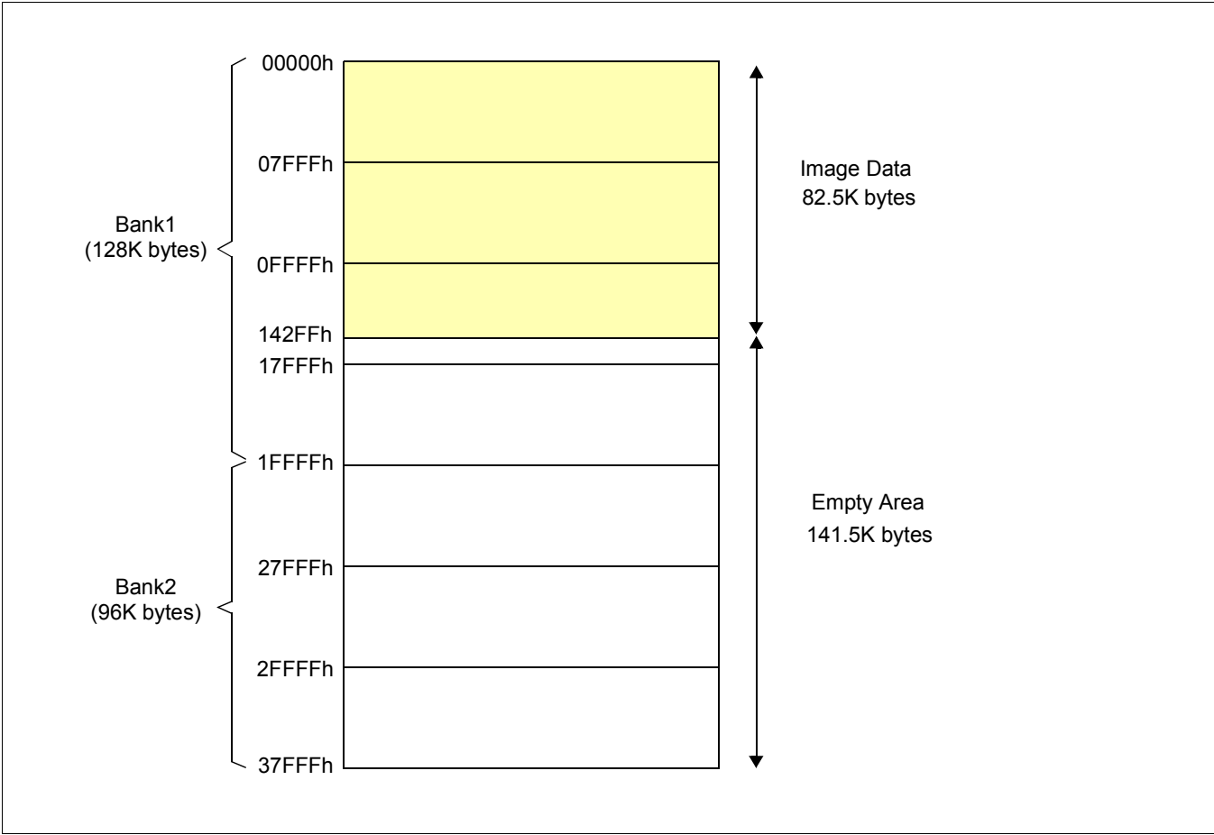
Figure 8-4: Memory Map for Main Window Case 2
