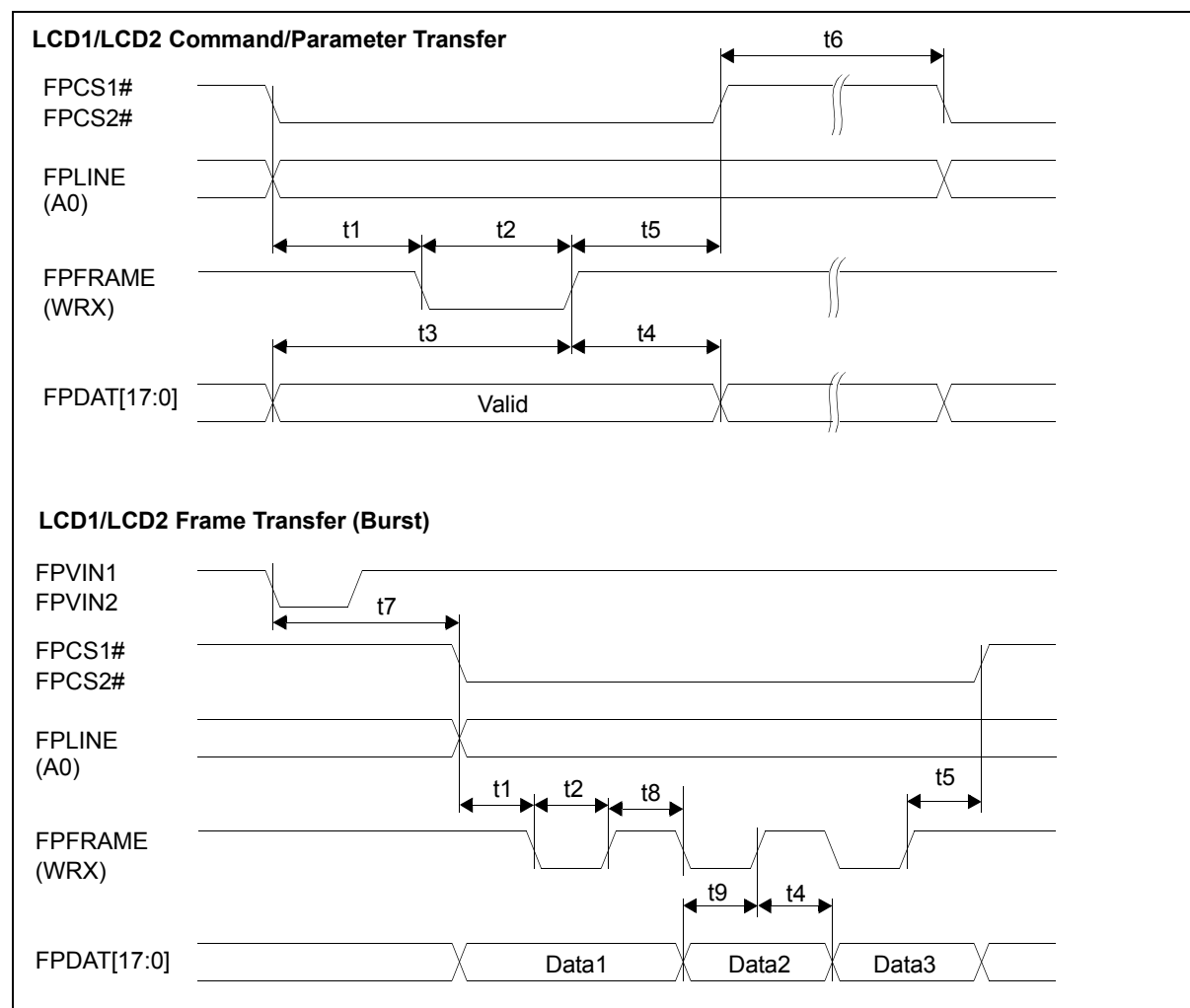
Figure 7-37: LCD1, LCD2 Parallel Interface Timing (80)
