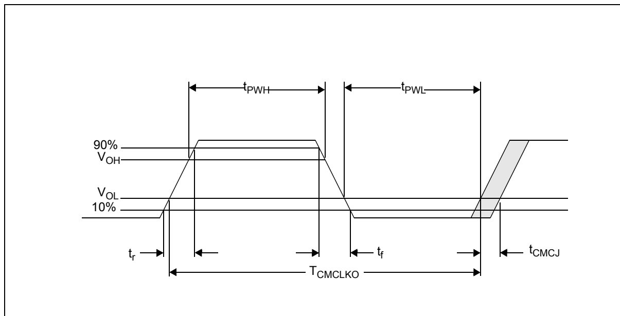
Figure 7-42: Camera Clock Output Timing
