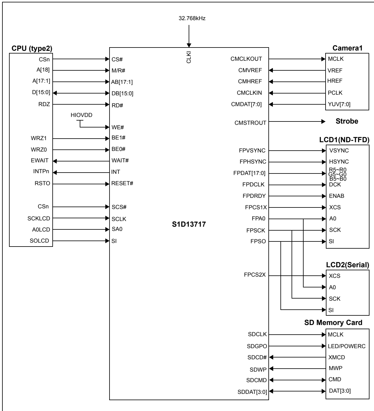
Figure 3-2: S1D13717 System Diagram 2
