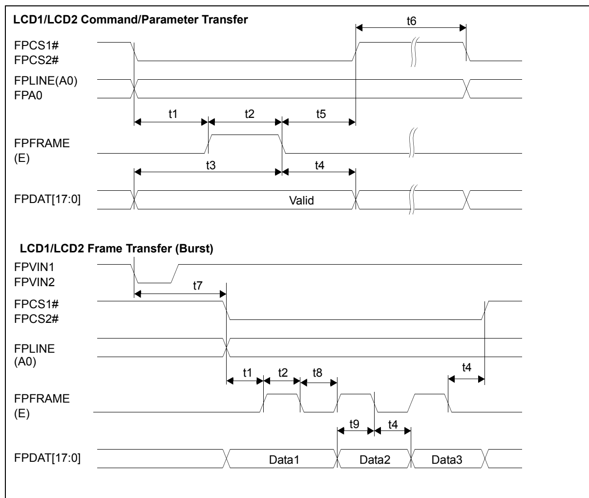
Figure 7-38: LCD1, LCD2 Parallel Interface Timing (68)
