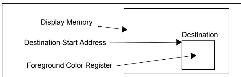
Figure 16-4: Solid Fill BitBLT Data Flow
