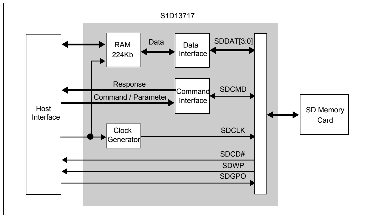
Figure 21-1: SD Memory Card Interface Block Diagram
