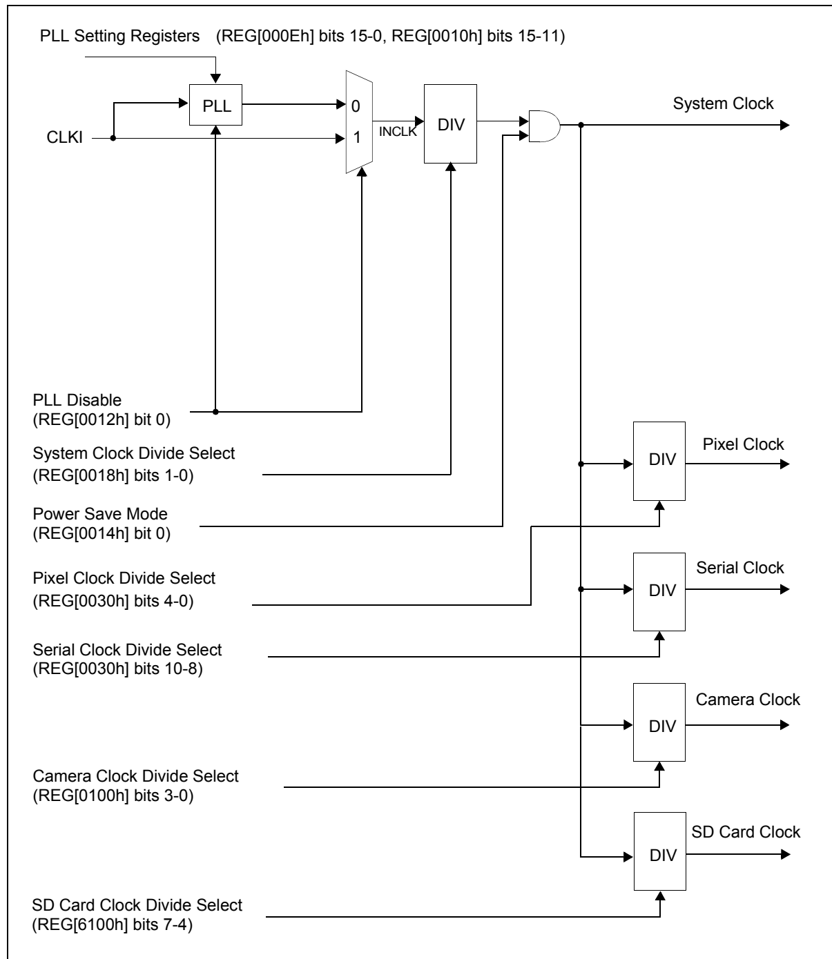
Figure 9-1: Clock Diagram
