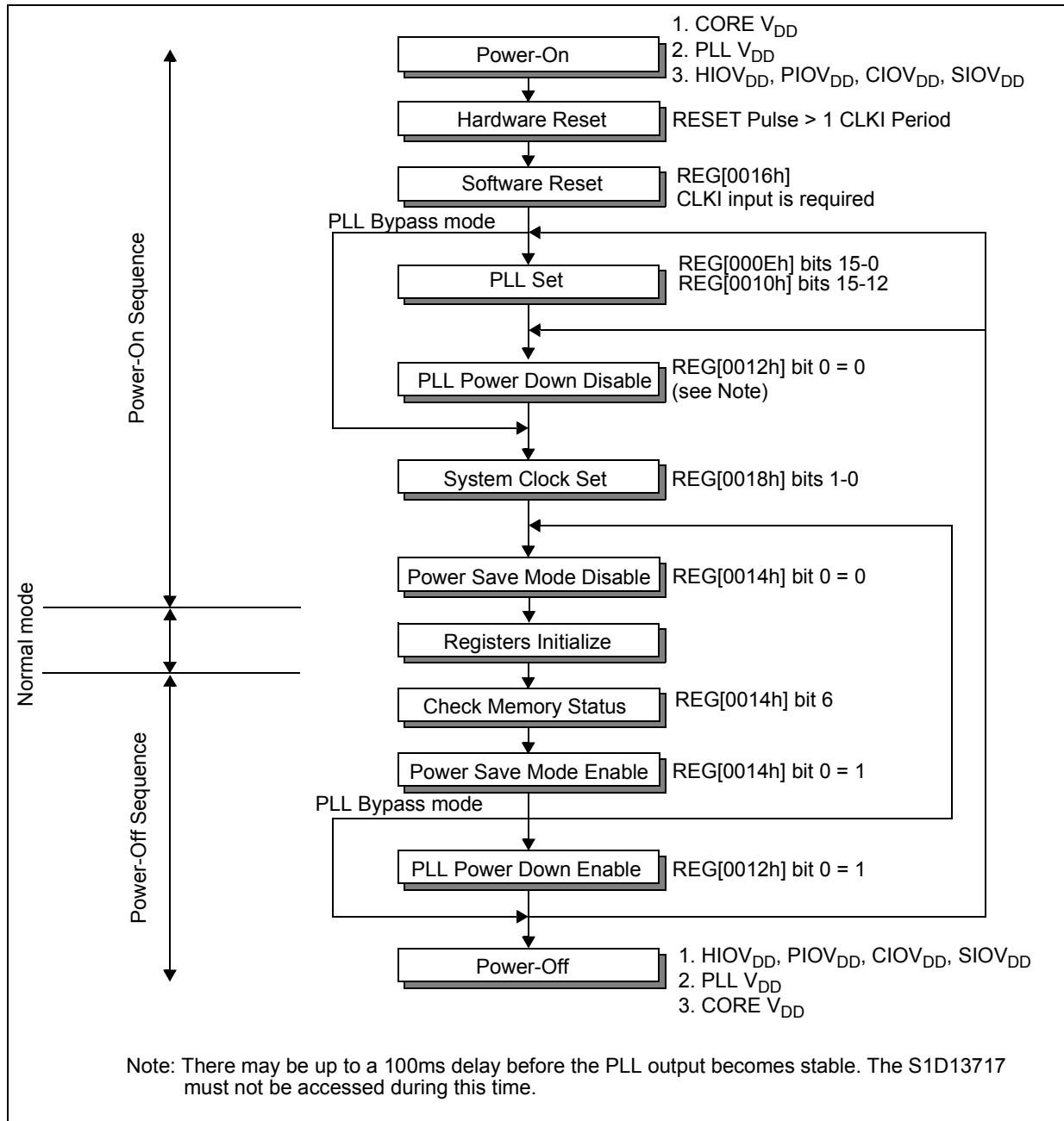
Figure 11-1: Power-On/Power-Off Sequence
