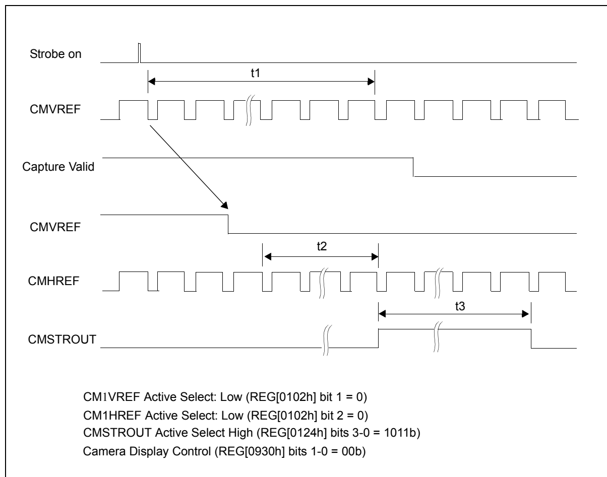
Figure 7-43: Strobe Control Output Timing
