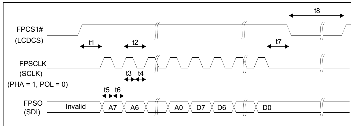
Figure 7-36: LCD1 uWIRE Serial Interface Timing
