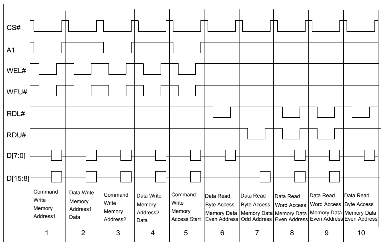
Figure 22-3: Memory Read Example Sequence
