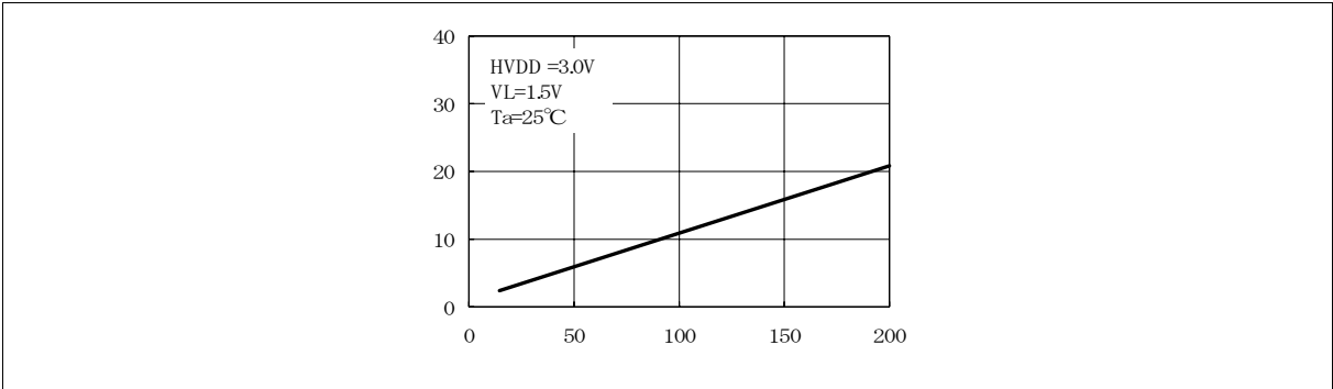
Figure 7-40: Fall Time V.s. Capacitance ( C_L )
