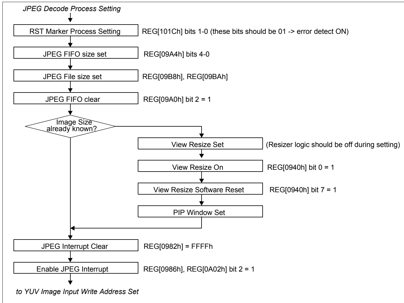
Figure 19-8: JPEG Decoding Process (3 of 6)
