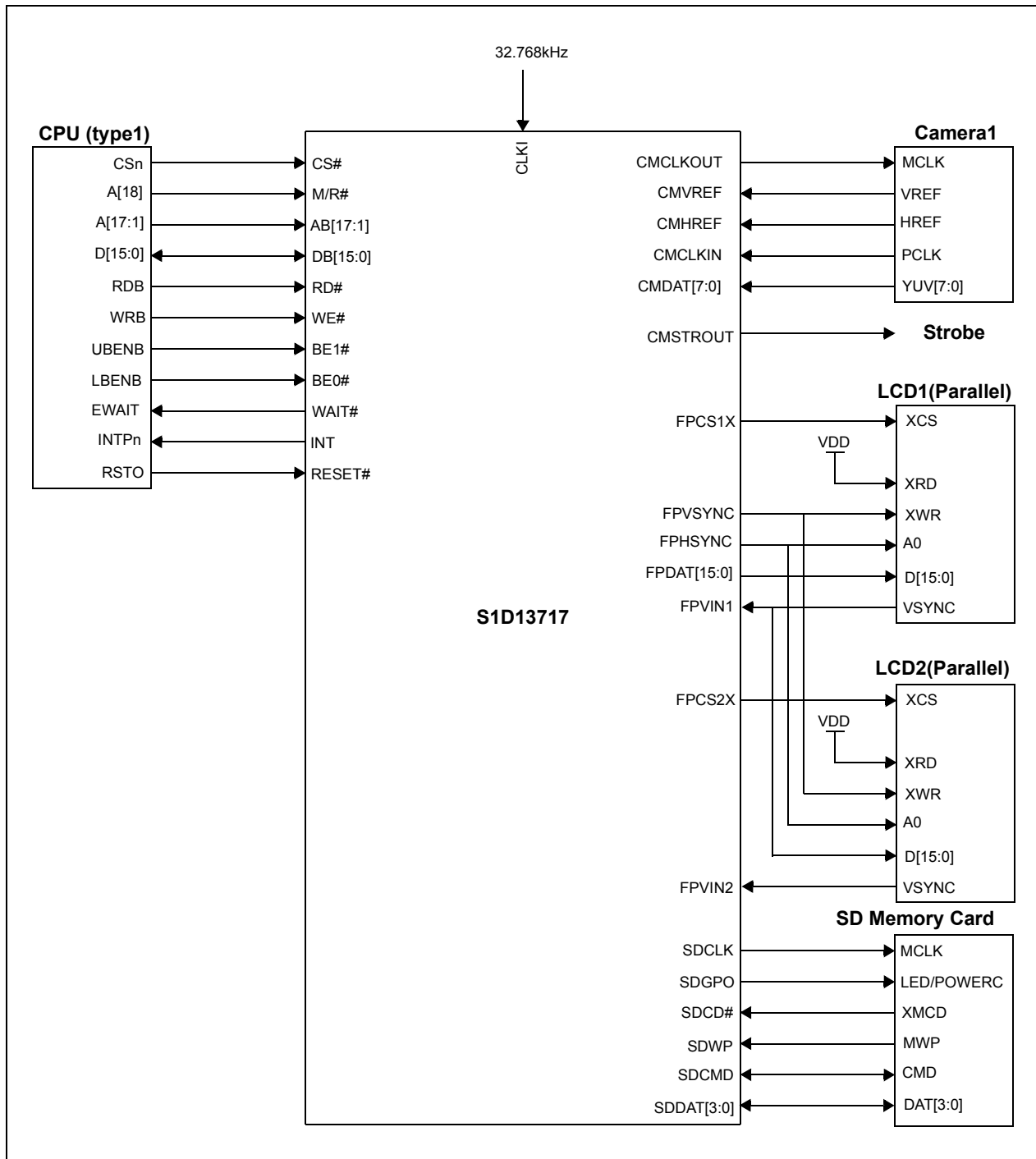
Figure 3-4: S1D13717 System Diagram 4
