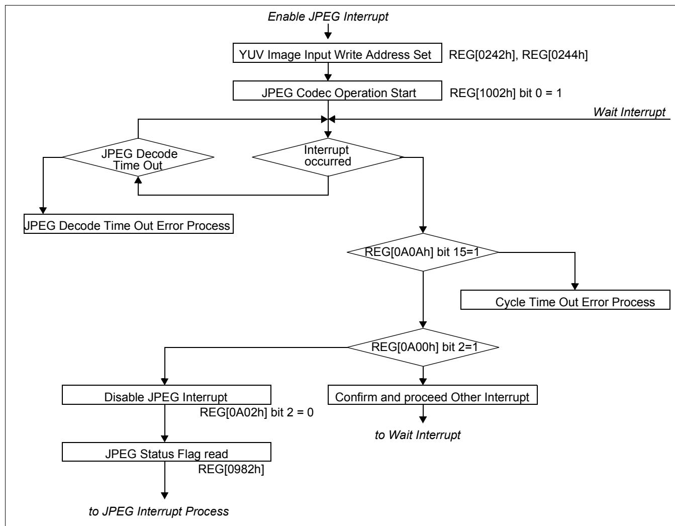
Figure 19-9: JPEG Decoding Process (4 of 6)
