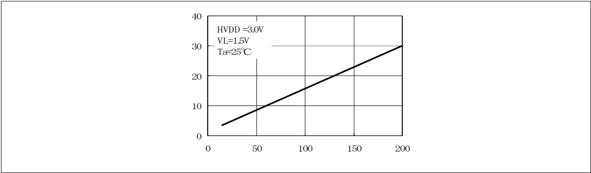
Figure 7-39: Rise Time v.s. Capacitance ( C_L )
