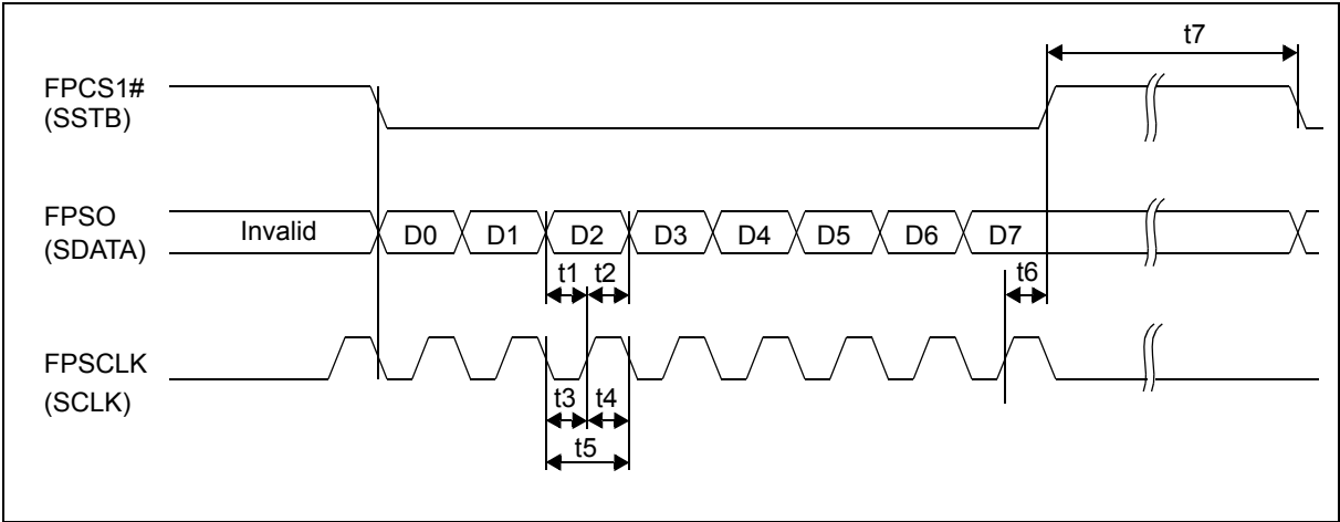
Figure 7-35: LCD1 a-Si TFT Serial Interface Timing
