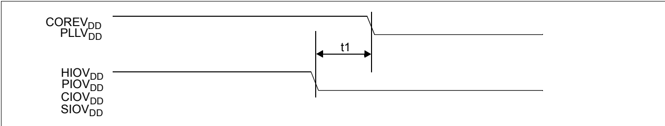
Figure 7-5: Power-Off Sequence
