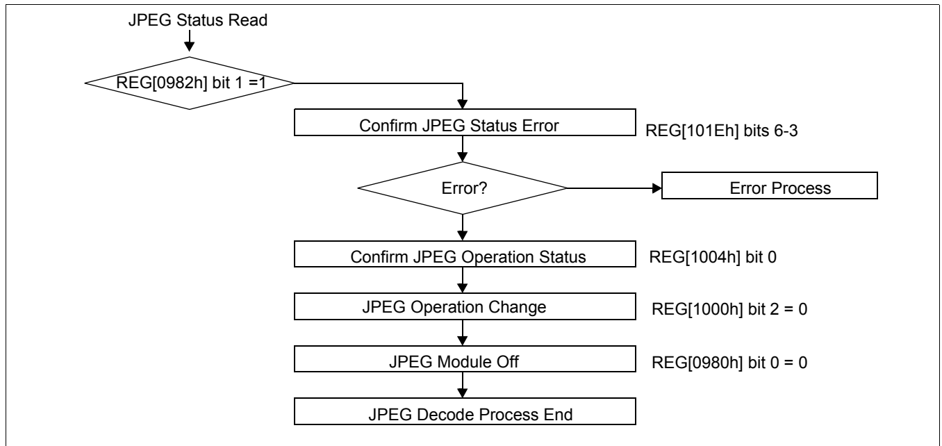
Figure 19-11: JPEG Decoding Process (6 of 6)
