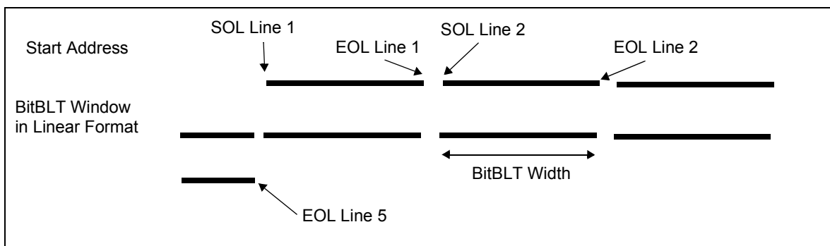
Figure 16-9: Memory Linear Example
