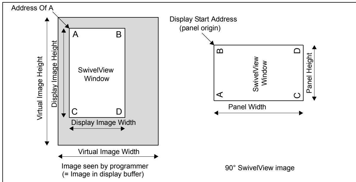
Figure 14-1: Relationship Between The Screen Image and the Image Refreshed in 90° SwivelView.
