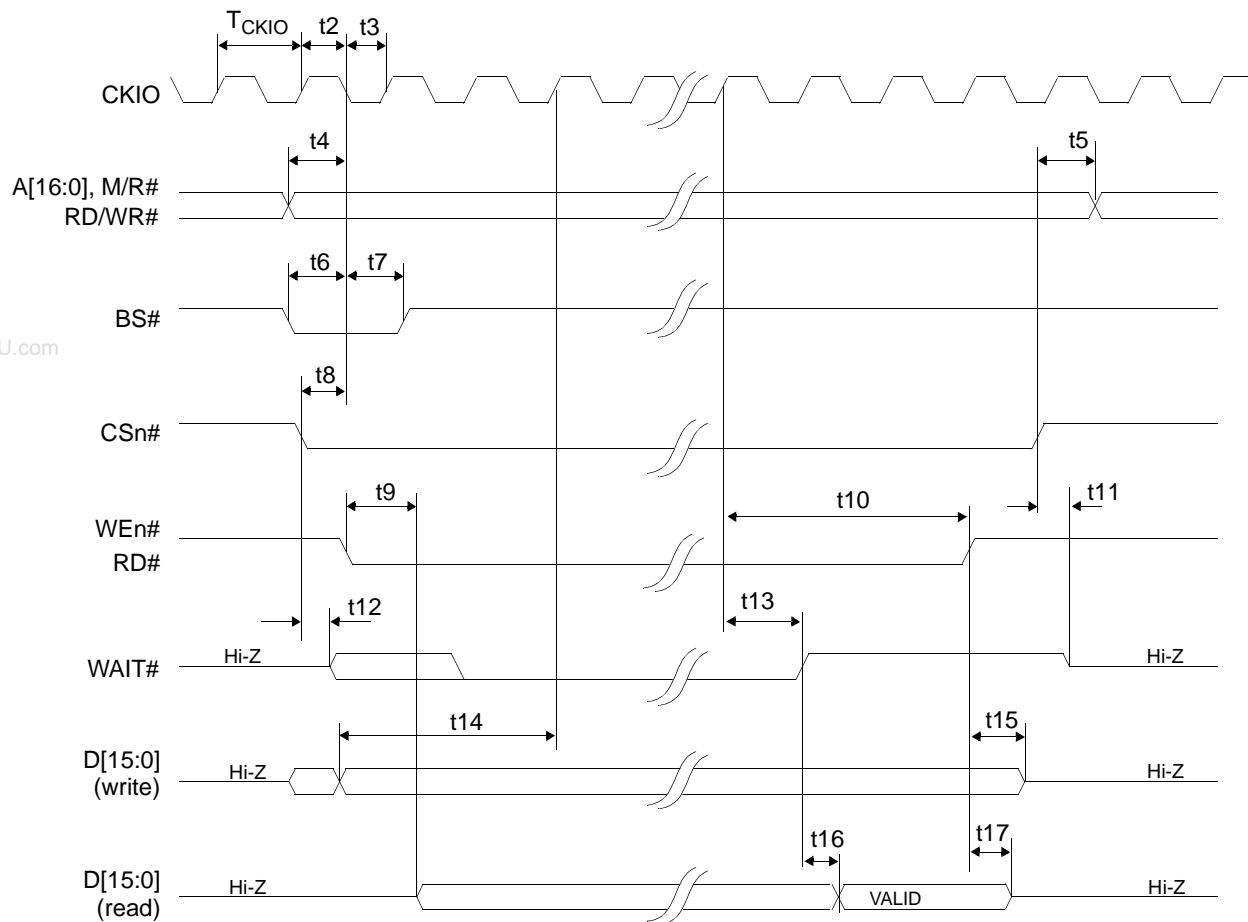
Figure 7-2: SH-3 Bus Timing
