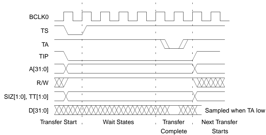
Figure 2-1: MCF5307 Memory Read Cycle
