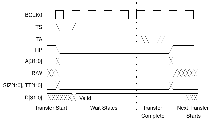
Figure 2-2: MCF5307 Memory Write Cycle
