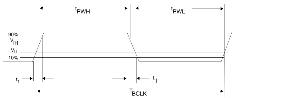
Figure 7-8: Clock Input Requirements for BCLK
