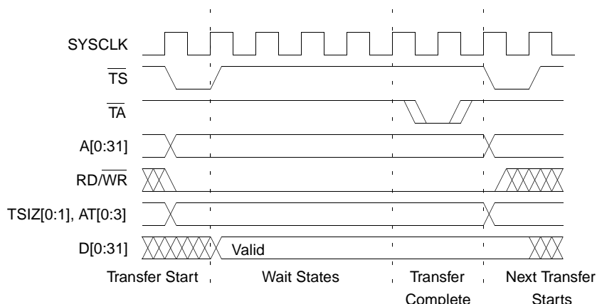
Figure 2-2: Power PC Memory Write Cycle
