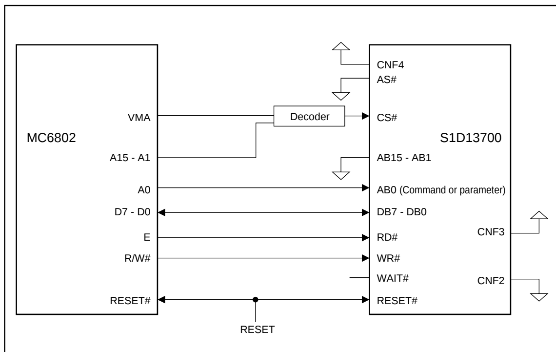
MC6802 System Block Diagram (Indirect)
