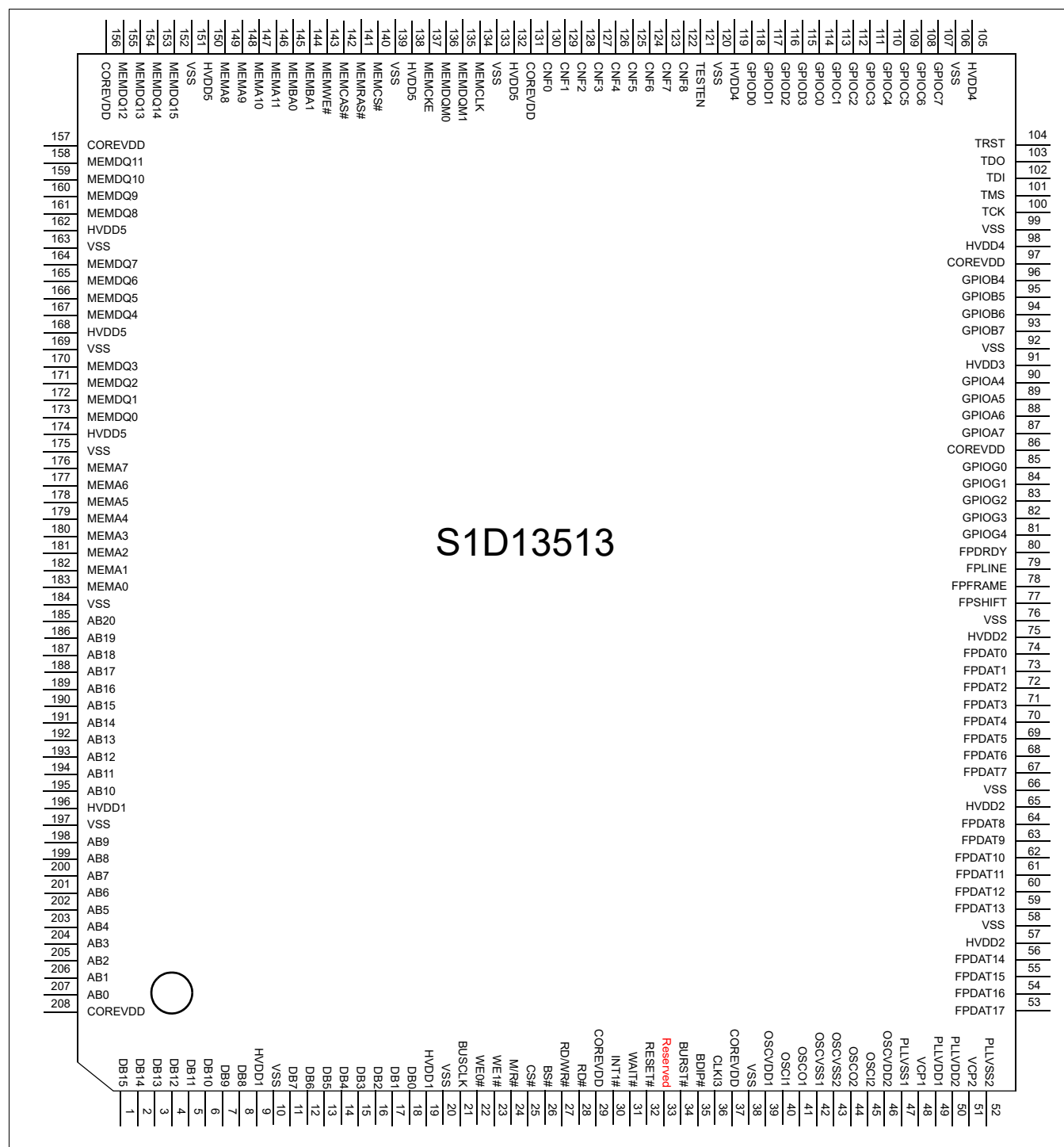
Figure 5-1: QFP22-208 Pinout
