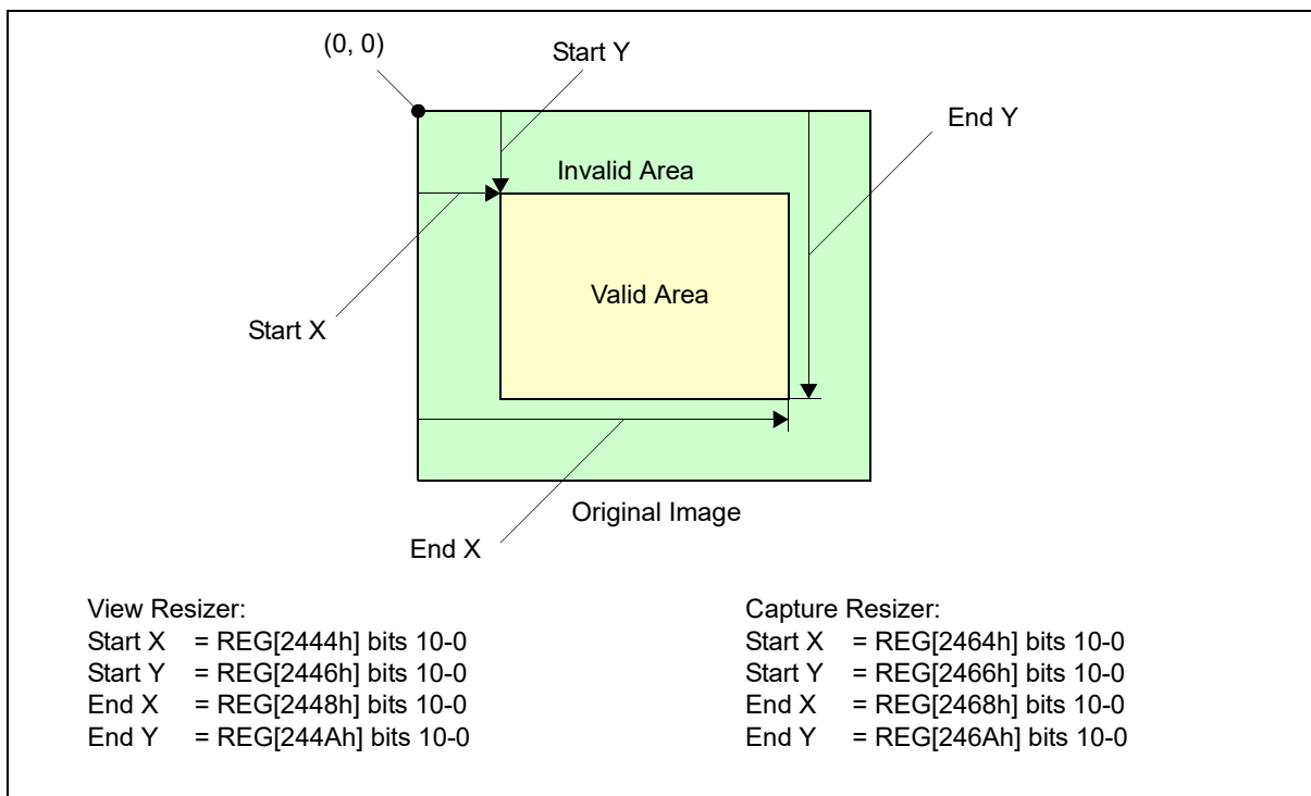
Figure 14-2: Trimming Function
