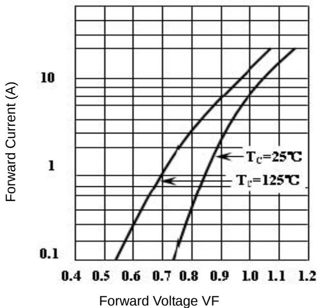
Fig.3 Forward Voltage
