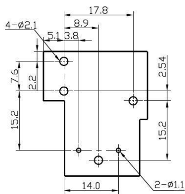
S12(P) type(2 common terminal)
