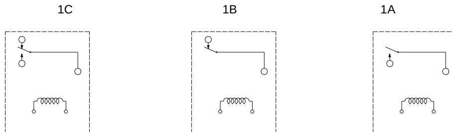
S12(Q) BOTTOM VIEW
