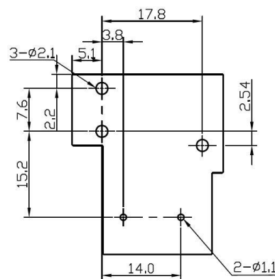
S12(P) type(1 common terminal)
