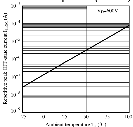
Fig.8-b Repetitive Peak OFF-state Current vs. Ambient Temperature (S208T01)
