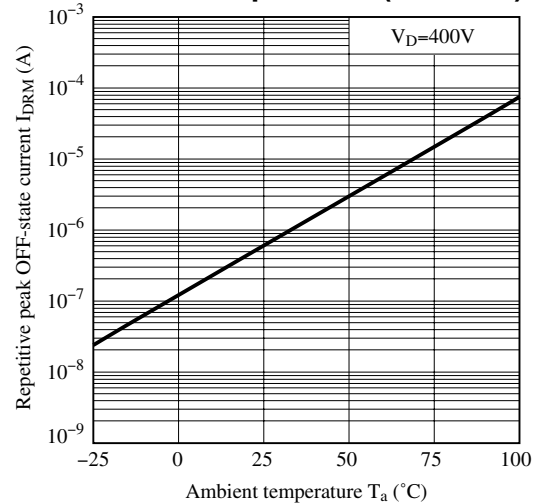
Fig.8-a Repetitive Peak OFF-state Current vs. Ambient Temperature (S108T01)
