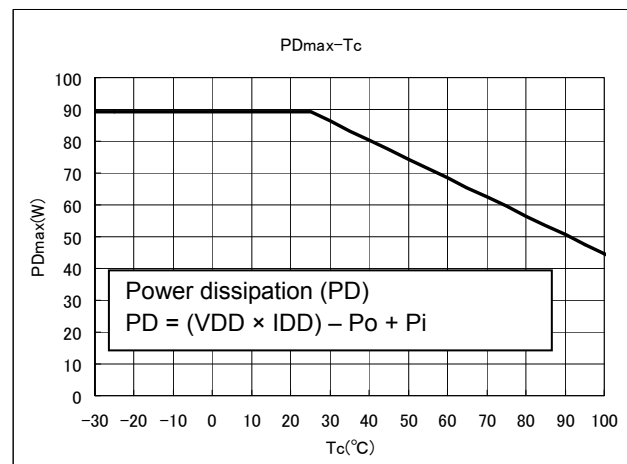
Figure 2 PDmax-Tc
