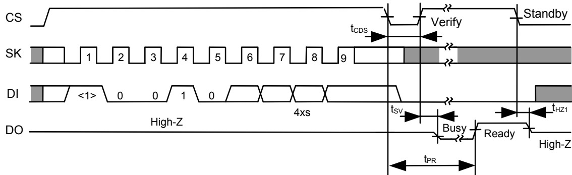
Figure 14 Chip Erase Timing (S-93C46C)
